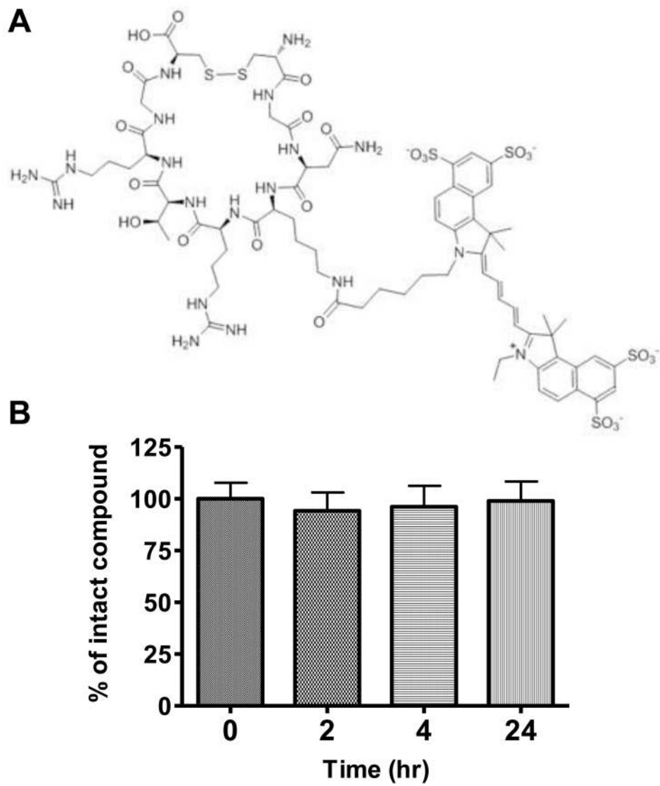
Figure 1. (A) Structure of Cy5.5-LyP-1. (B) Serum stability of Cy5.5-LyP-1 with LC-MS.
