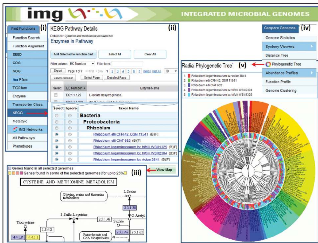
Figure 4. Comparative analysis tools. (i) A pathway is selected from the list of KEGG pathways via the KEGG option of the 'Find Functions' menu, and subsequently (ii) the 'KEGG Pathway Details' lists its associated enzymes and the list of genomes organized phylogenetically. (iii) Once genomes are selected for comparison, the result is displayed in the context of the KEGG pathway map, with each enzyme number on the map coloured depending on the percentage of genomes with a gene associated with that enzyme. (iv) The 'Radial Phylogenetic Tree' is one of several tools provided for comparing genomes, and (v) allows comparing the BLAST hits of the genes of up to five user selected genomes to the genes of all the genomes in the database using a colour-coded hierarchical circular tree viewer.
