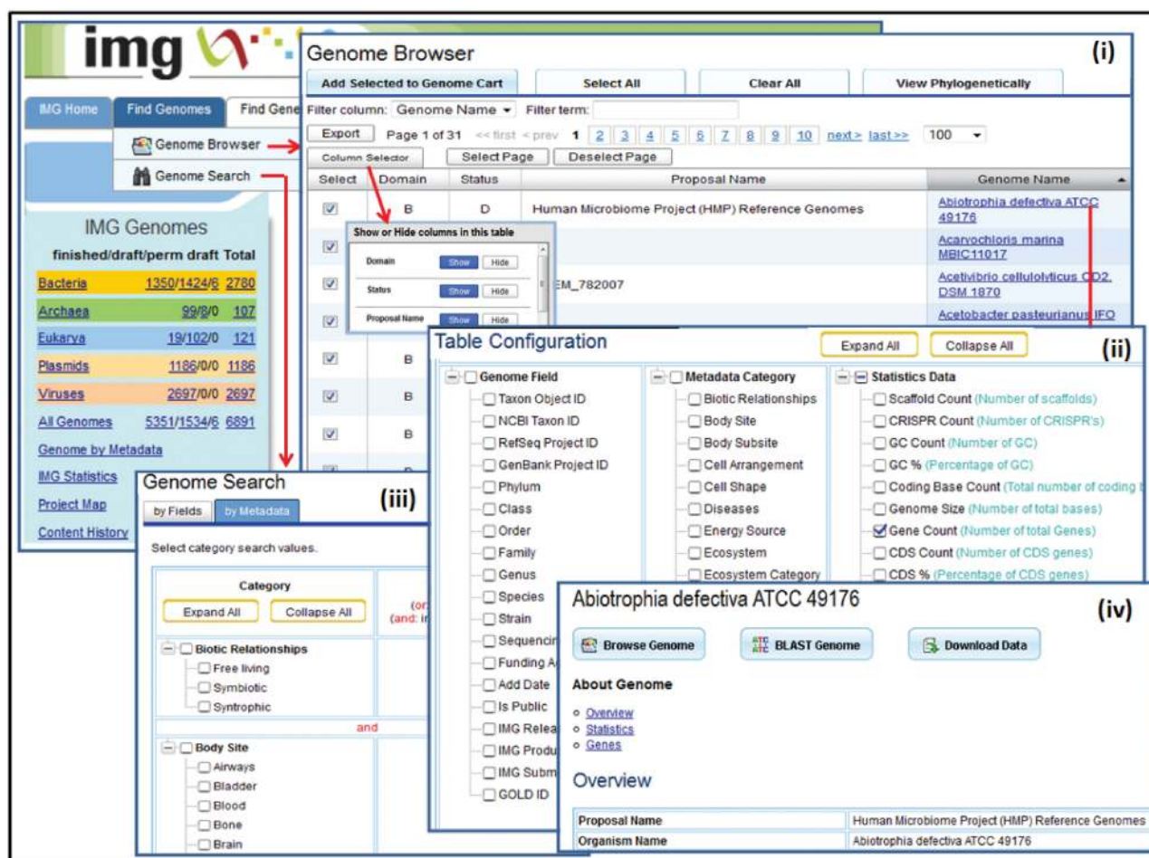
Figure 2. Genome browser and search tools. The 'Genome Browser' displays the genomes organized in a phylogenetic tree or (i) in a tabular list that can be configured by (ii) adding or removing genome, metadata or annotation specific columns. (iii) 'Genome Search' allows searching genomes on genome or metadata specific fields. (iv) A genome can be explored using a variety of browsing tools, searched for the presence of specific genes using BLAST, or downloaded.
