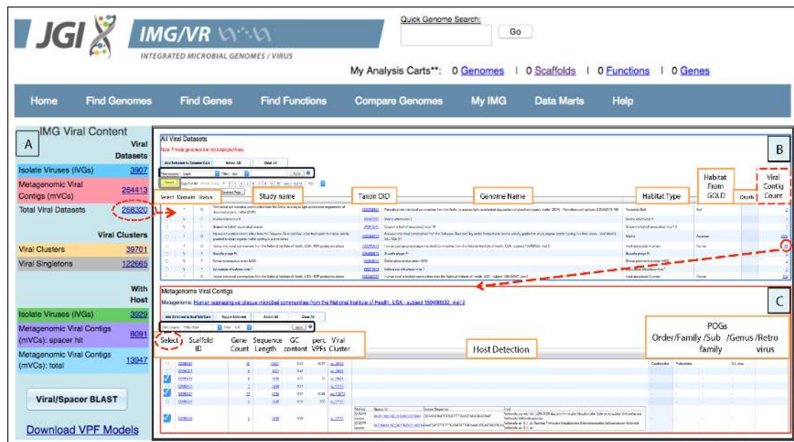
Figure 2. Browsing IMG/VR viral datasets. (A) Total counts and access to the list of viral sequences from isolate viruses, metagenomic viral contigs, or their combination (dashed red oval). (B) Detailed table from 'Total Viral Datasets' link displaying study and sample name, Taxon OID, habitat information and number of metagenomic viral contigs. (C) List of viral metagenomic contigs found in a single sample. Columns in (B) and (C) can be sorted by clicking on the column header, and different filters can be used for specific searches (black boxes). Tables can be also exported in a tab-delimited text format by using the Export button (grey box with yellow background).
