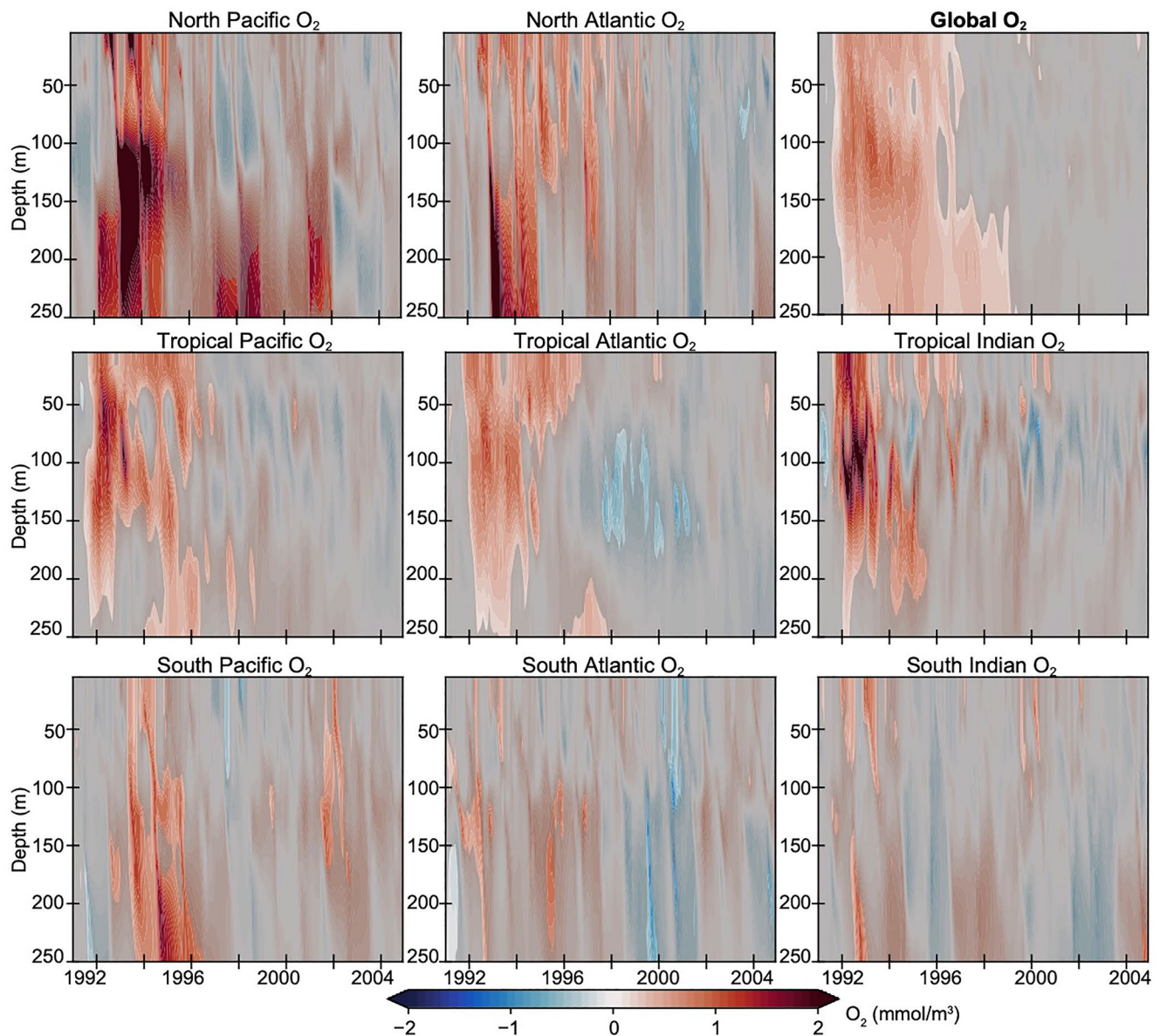
Figure 6. Regionally averaged vertical profile of difference (Community Earth System Model Large Ensemble [CESM-LE] minus CESM-LE-NoPin) plots for ensemble mean O_2 inventory ( \text{mmol m}^{-3} ). Separations are made for the Pacific, Atlantic, and Indian basins into northern ( >30^\circ\text{N} ), tropical ( 30^\circ\text{N} – 30^\circ\text{S} ), and southern sections ( <30^\circ\text{S} ) while the global profile is shown in the top right panel. Shading indicates time/depth where differences are not significant at the 95% confidence level (Deser, Phillips, Bourdette, & Teng 2012). Positive anomalies (warm colors) indicate greater oxygen inventory values with the eruption of Pinatubo while negative anomalies (cool colors) indicate lower oxygen with the eruption. Similar plot with depth extending to 1,000 m is available in Figure S8 in Supporting Information S1.
