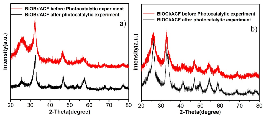
Fig. S6. XRD patterns of BiOBr/ACF (a) and BiOCl/ACF (b) after photodegradation
