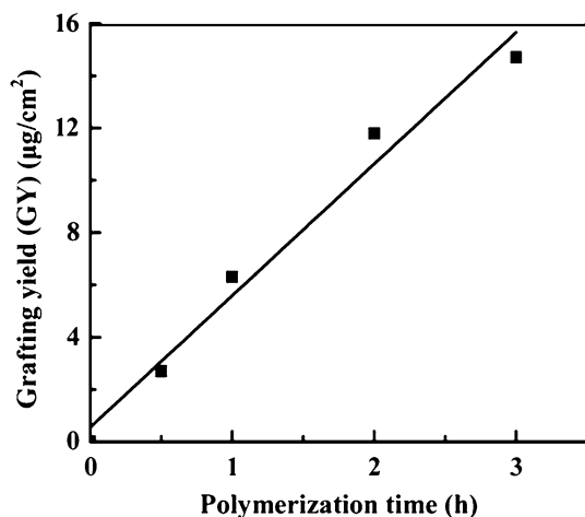
Fig. 5 A linear relationship between the grafting yield (GY) of the P(GMA) brushes with the surface-initiated ATRP time was observed. The polymer chain growth from the PCL-Br surface could be controlled by varying reaction time
