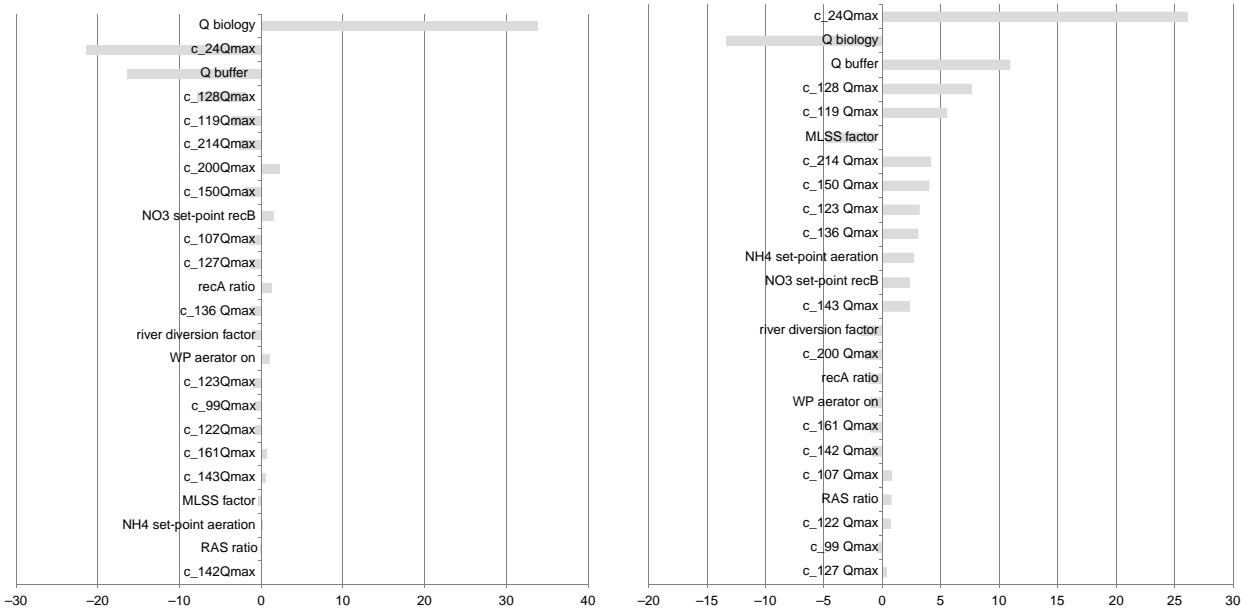
Figure 11. Example of GSA results; regression coefficients (as % of total sensitivity) ranking the sensitivity of operational parameters on the minimum DO (left) and maximum NH 4 (right) in the closing river section for the small storm.
