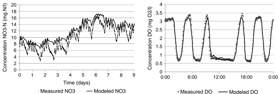
Figure 4. Performance of WWTP model: nitrate in effluent (left) and DO in aeration tank (right).
