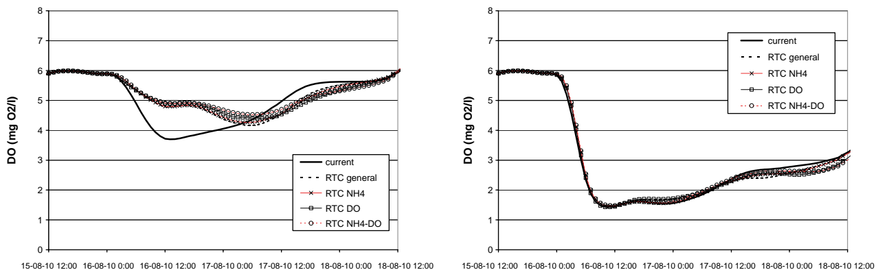
Figure 13. Impact of applying RTC strategies on DO concentration in the Dommel River downstream of Eindhoven for a small storm event (left) and for a large storm event (right).
