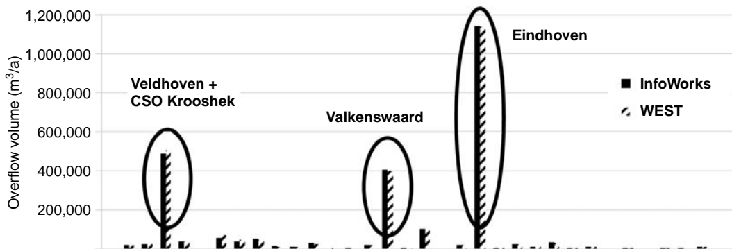
Figure 8. Comparison of annual overflow volumes from the main CSOs in the sewer system, produced by the detailed InfoWorks model and by the simplified WEST model.
