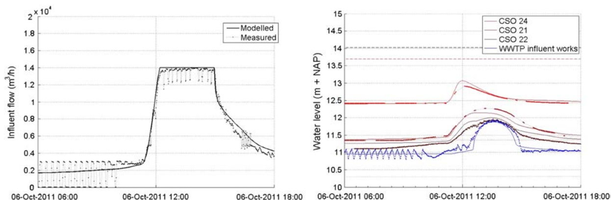
Figure 2. Pumped flow ( m^3/h ) from Eindhoven at influent works (left) and water level (m + NAP) at influent works and three upstream CSOs (number 21, 22 and 24) (right) for storm event 6 October 2011. Dotted lines are monitoring data, solid lines model results.
