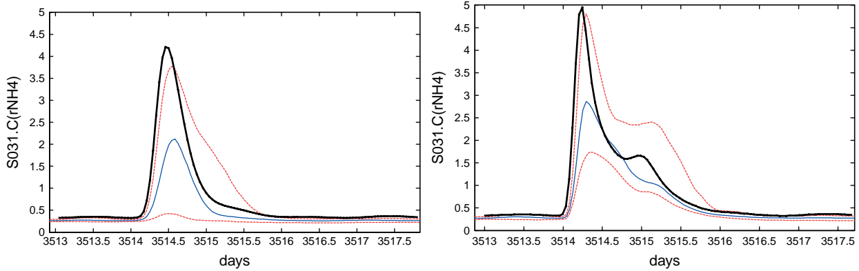
Figure 10. (Colour online) Example of GSA results; X-axis time in days and Y-axis NH 4 concentration in mg/L in the closing river section, with 0.075-y -1 storm (left) and 5-y -1 storm (right); the red lines are the 5th and 95th percentiles, the blue line is the median, the black line the current situation.
