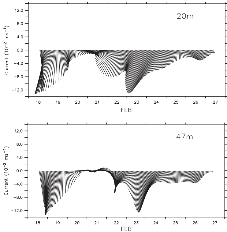
Fig. 9. Stick diagram of current meter measurements (cm/s; one stick every hour) at the mooring array located at the 80 m isobath (see Fig. 1 for location) from 18 to 27 February 2000: (a) current meter located at the 20 m depth level, and (b) current meter located at the 47 m depth level. Negative values correspond to equatorward currents.
