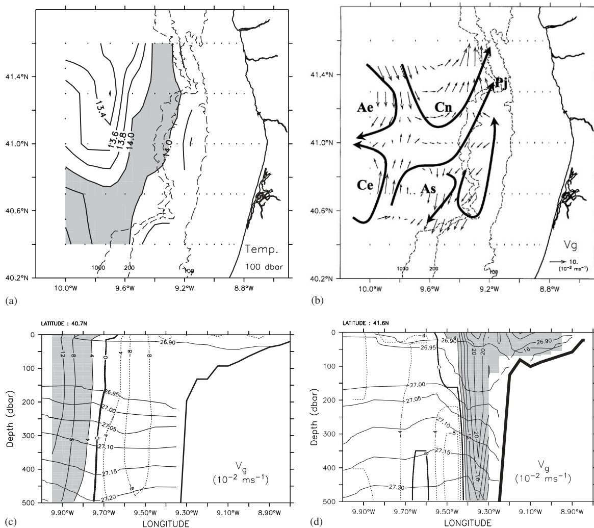
Fig. 3. Horizontal distributions of (a) temperature at 100 dbar ( ^{\circ}\text{C} ; values >14^{\circ}\text{C} are in shaded) and (b) geostrophic velocity ( \text{cm/s} ) referred to 1350 dbar at 100 m depth, and vertical fields of geostrophic velocity ( \text{cm/s} ) referred to 1350 dbar superimposed in density fields ( \sigma_t ) for (c) section II ( 40.7^{\circ}\text{N} ) and (d) section V ( 41.6^{\circ}\text{N} ). Poleward flow is shaded in vertical fields. Cn and Ce represent cyclonic eddies, Ae and As represent anticyclonic eddies, and Pj is the poleward slope jet (see text for details).
