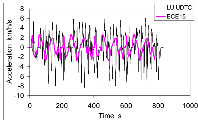
Figure 5 Comparison of accelerations and decelerations between LU-UDTC and ECE15 test cycles
