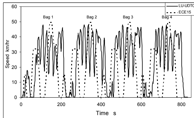
Figure 4 Typical road speed profile of LU-UDTC cycle
