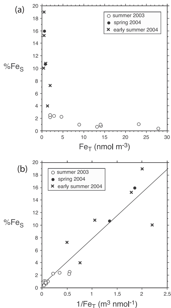
Figure 3. (a) Operational solubility of aerosol iron ( \%Fe_S ) versus total aerosol iron concentration ( Fe_T ) for FeATMISS aerosol samples; (b) \%Fe_S versus 1/Fe_T for the same samples, showing best fit linear regression ( r^2 = 0.85 ). Open circles, summer 2003 cruise; filled circles, spring 2004 cruise; crosses, early summer 2004 cruise.
