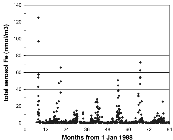
Figure 5. Time series record of total aerosol iron concentrations at Tudor Hill, Bermuda, for the period 1988–1994 (data provided by S. Huang). The summertime concentration maxima are typically associated with the transport of North African (“Saharan”) dust to the Bermuda region.
