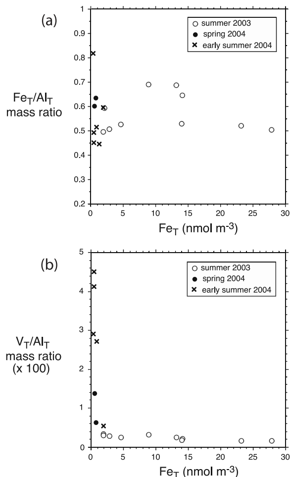
Figure 7. Mass ratios of (a) \text{Fe}_T/\text{Al}_T and (b) \text{V}_T/\text{Al}_T plotted against total iron concentration for FeATMISS aerosol samples. Open circles, summer 2003 cruise; filled circles, spring 2004 cruise; crosses, early summer 2004 cruise.
