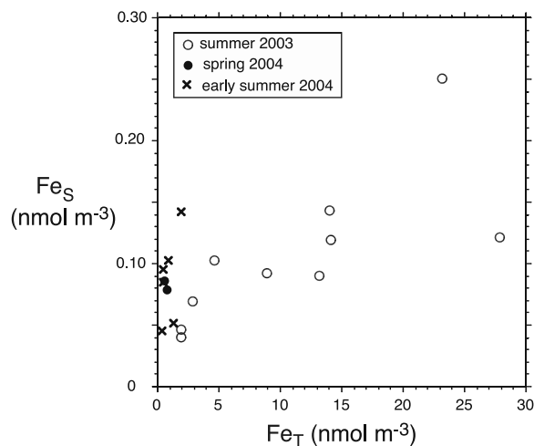
Figure 10. Atmospheric concentration of operationally defined soluble aerosol iron ( Fe_S ) versus total aerosol iron concentration ( Fe_T ) for FeATMISS aerosol samples. Open circles, summer 2003 cruise; filled circles, spring 2004 cruise; crosses, early summer 2004 cruise.
