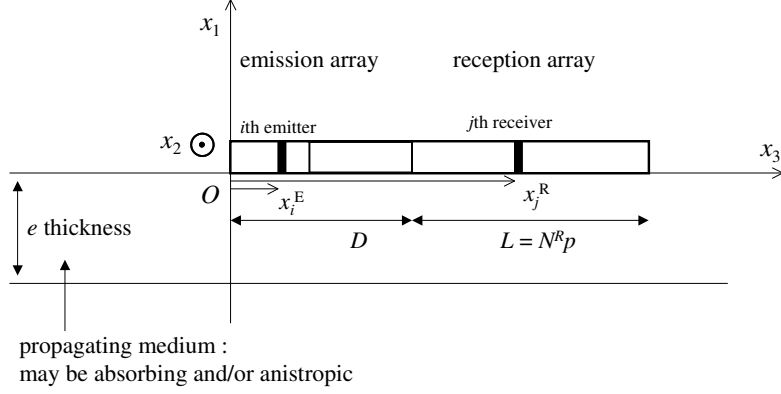
FIG. 1. Geometry of the problem: emission and reception arrays are placed in the axial transmission configuration.
