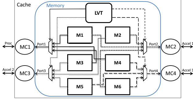
Figure 2. LVT-based 4-ported cache.
