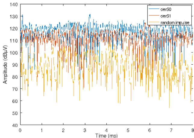
FIGURE 7. der50, der51 and random impulsive noises in-band power representation in time with a resolution of 50 μs.
