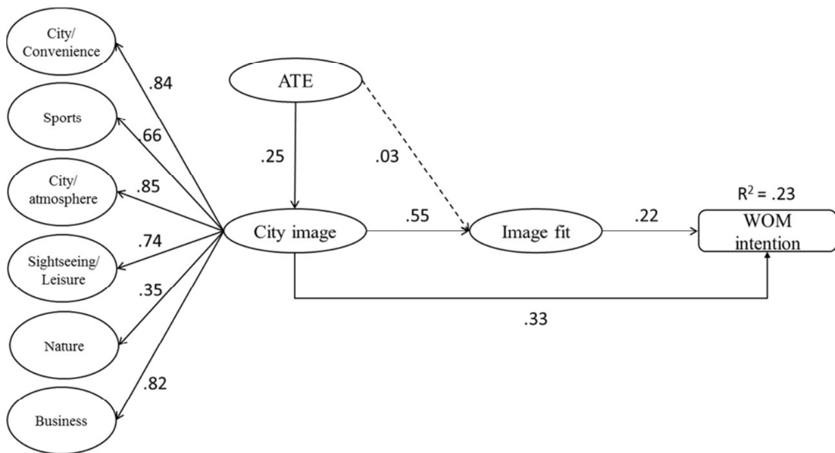
Figure 2. Results of the structural equation modeling ( \chi^2/df = 2.48 , CFI = .900, TLI = .900, RMSEA = .074).
