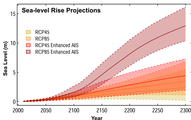
Fig. 4. Sea-level projections from 2010 to 2300. Projections are calculated using RCP4.5 (yellow) and RCP8.5 (orange) projections (21) and for projections combining AIS contributions from ref. 26 with the RCP4.5 (red) and RCP8.5 (dark red) projections from ref. 21. Lines and shaded regions represent the median and the central 95% credible interval.
