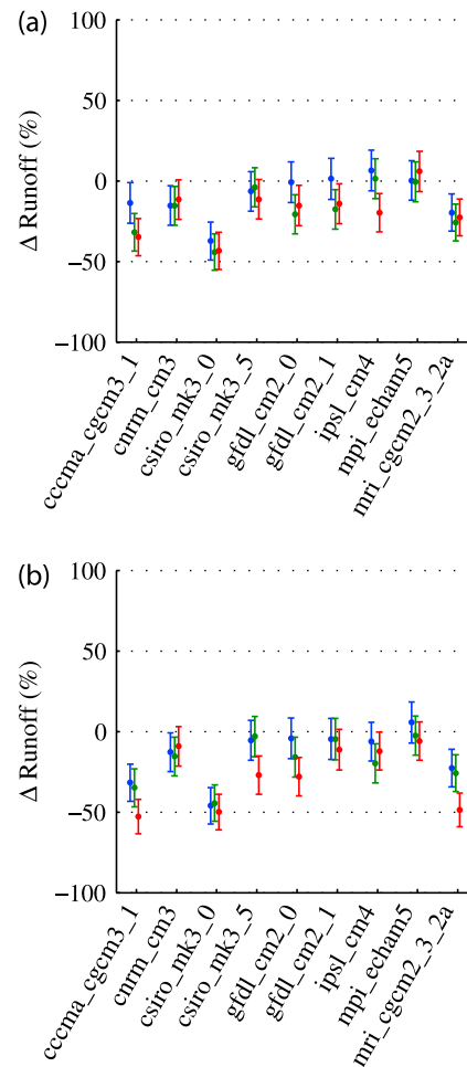
Figure 8. Projected changes in wet season runoff in the Gilgel Abay River compared to the base period 1980–2000, calculated with the SWAT model: (a) changes to 2046–2065 and (b) changes to 2080–2100. Colors denote the SRES scenario used: blue, B1; green, A1B; red, A2. Changes are expressed as percentages of the base period (1980–2000) wet season runoff.
