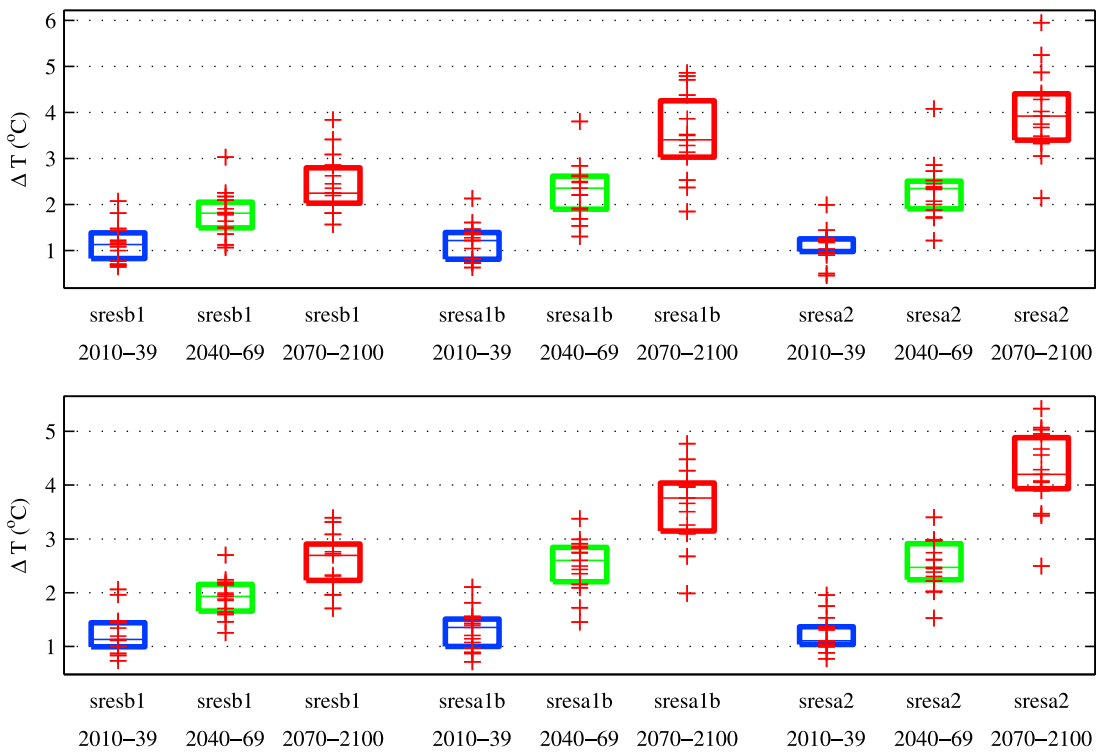
Figure 4. Projected changes in mean temperature at the location of Adet station for three SRES scenarios and time periods, calculated from monthly GCM outputs: (top) changes in wet season temperature and (bottom) changes in dry season temperature. The results for the individual GCMs are shown as pluses, and the boxes show the 25th, 50th, and 75th percentiles.
