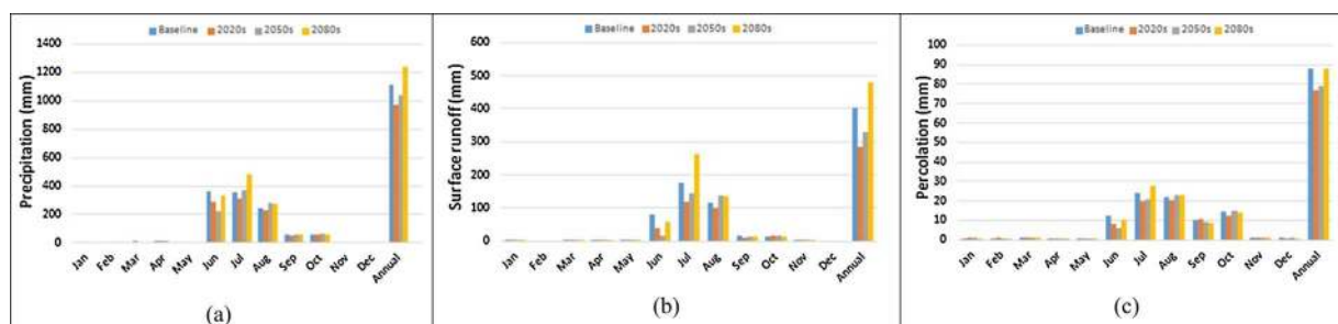
Fig. 8. Average condition: PRECIS q1 projection impact on changes in absolute magnitude of (a) precipitation, (b) surface runoff, and (c) percolation.
