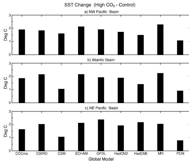
FIG. 2. SST change (high \text{CO}_2 - control) in ^{\circ}\text{C} for each CMIP2+ climate model (bottom axis label) for the (a) NW Pacific, (b) Atlantic, and (c) NE Pacific basins. This represents the warming that occurs in the tropical storm basins and tropical storm seasons over an 80-yr period during which atmospheric \text{CO}_2 concentrations increase at 1\% \text{ yr}^{-1} compounded in the model. See text for further details.
