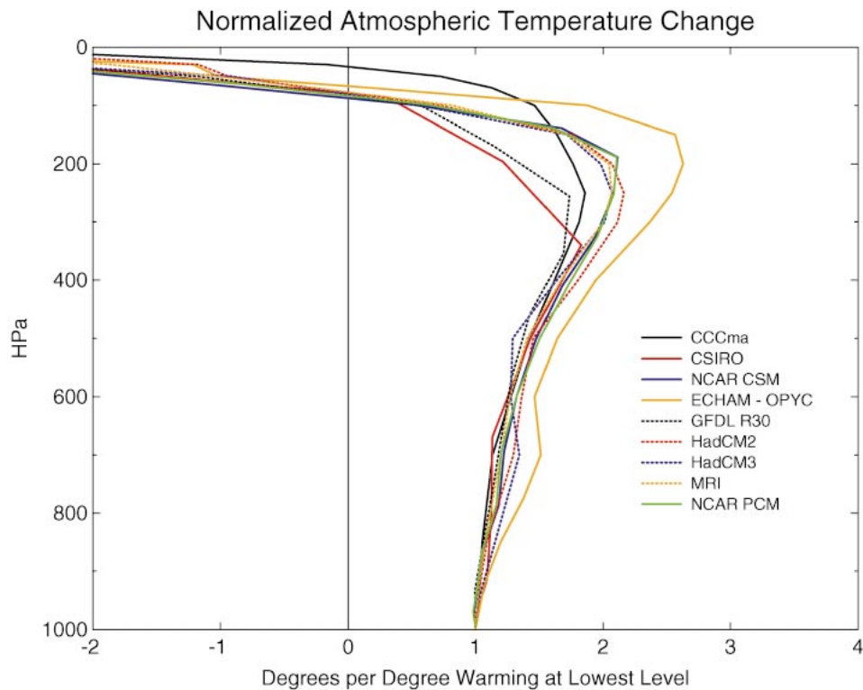
FIG. 3. Normalized atmospheric temperature change (high \text{CO}_2 - control) vertical profiles, zonally averaged over all latitudes from 20^{\circ}\text{N} to 20^{\circ}\text{S} . The difference is based on years 61–80 of the high \text{CO}_2 run minus years 61–80 of the control run for each CMIP2+ model (legend). The difference at each model level is normalized by dividing by the difference at the lowest level for that model.
