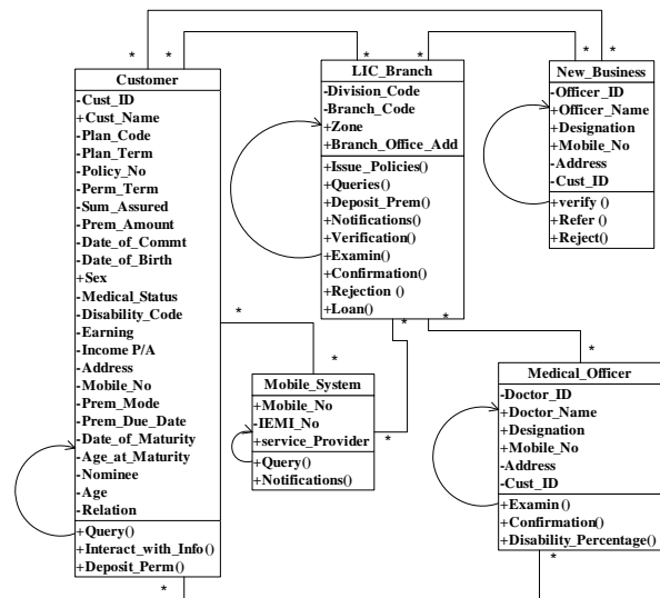
Figure 4. Attribute calling graph.
