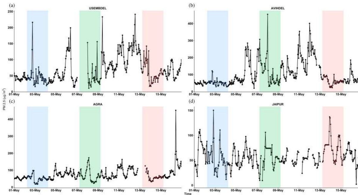
Figure 8. Changes in PM_{2.5} ( \mu g/m^3 ) recorded from four ground stations, during the three dust events. The ground stations shown are from (a) U.S. Embassy Delhi (USEMBDEL); (b) Anand Vihar, Delhi (AVIHDEL); (c) Agra; and (d) Jaipur. The U.S. Embassy in Delhi maintains the USEMBDEL station while the other three stations located in Anand Vihar, Delhi; Agra; and Jaipur are maintained by Central Pollution Control Board, India. The shaded areas represent the duration of the three dust events: blue, DE1; green, DE2; and red, DE3.
