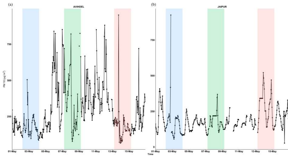
Figure 9. Changes in \text{PM}_{10} ( \mu\text{g}/\text{m}^3 ) recorded for (a) a station located in Anand Vihar, Delhi (AVIHDEL), and in (b) Jaipur. The shaded areas represent the duration of the three dust events: blue, DE1; green, DE2; and red, DE3.
