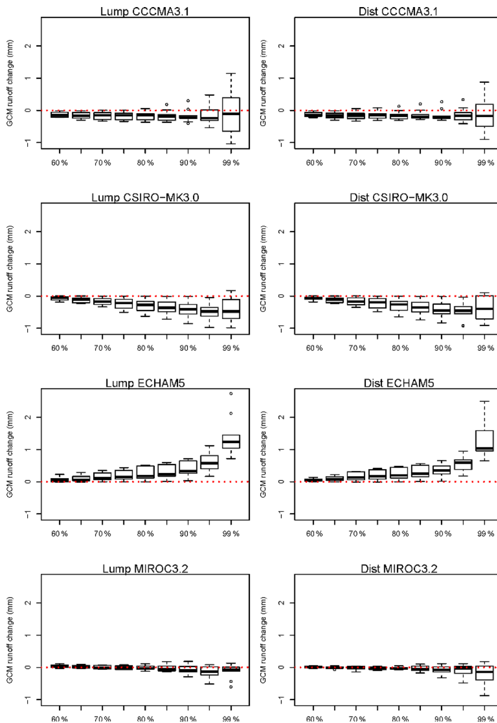
Figure 10. Simulated climate change runoff high-flow percentile changes (future minus historical using WRF-BC rainfall) of the 60th to 99th daily percentiles for lumped (left) and distributed (right) simulations. Box plots show the range across the 10 catchments.
