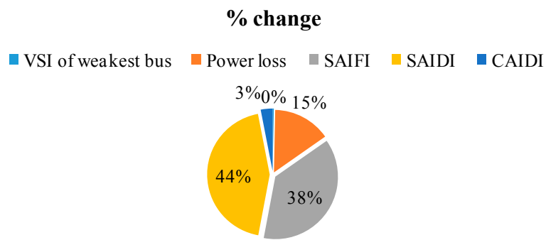
Figure 12. Comparative analysis of placement of charging station on VSI, power loss and reliability indices for Case 4.
