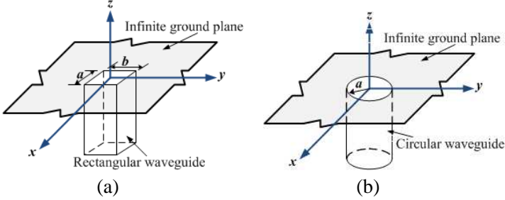
Figure 2. Geometry of (a) rectangular and (b) circular waveguides mounted on an infinite ground plane.
