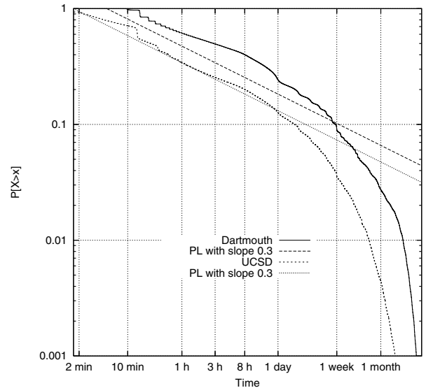
Fig. 2. Tail distribution function of the inter-contact time: data collected in Dartmouth and UCSD.
