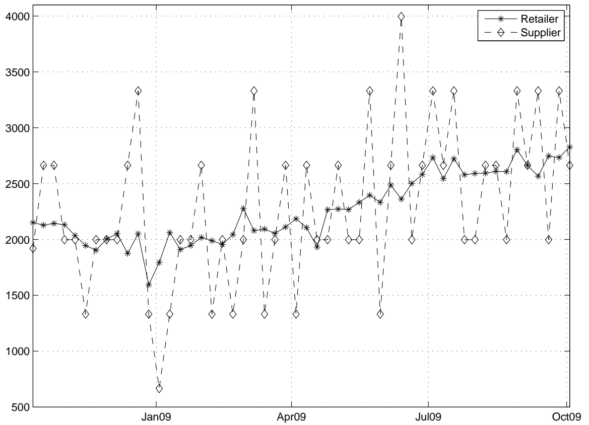
Figure 2: Example of a typical SKU. Retailer sales are in a solid line (-) and Volume received in a dashed line (- -)
