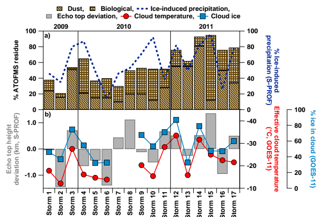
Figure 4. Summary of IN precipitation residue composition, observed surface meteorology at SPD, and cloud properties above SPD. (a) The percentages of dust and biological residues and the % ice-induced precipitation (snow plus BB rain). (b) Echo top height deviation (km) calculated from all storms during CalWater (average: 3.51 km based on data from 43 days during ATOFMS sample collection time periods provided in Table 1). Positive (negative) deviations correspond to higher (lower) than average echo top heights. Effective cloud temperature and percentage of cloud ice are also shown. Data were removed if in the homogeneous nucleation regime ( \leq -36^\circ\text{C} ). The respective instruments in which each measurement was acquired is provided in the axis labels.
