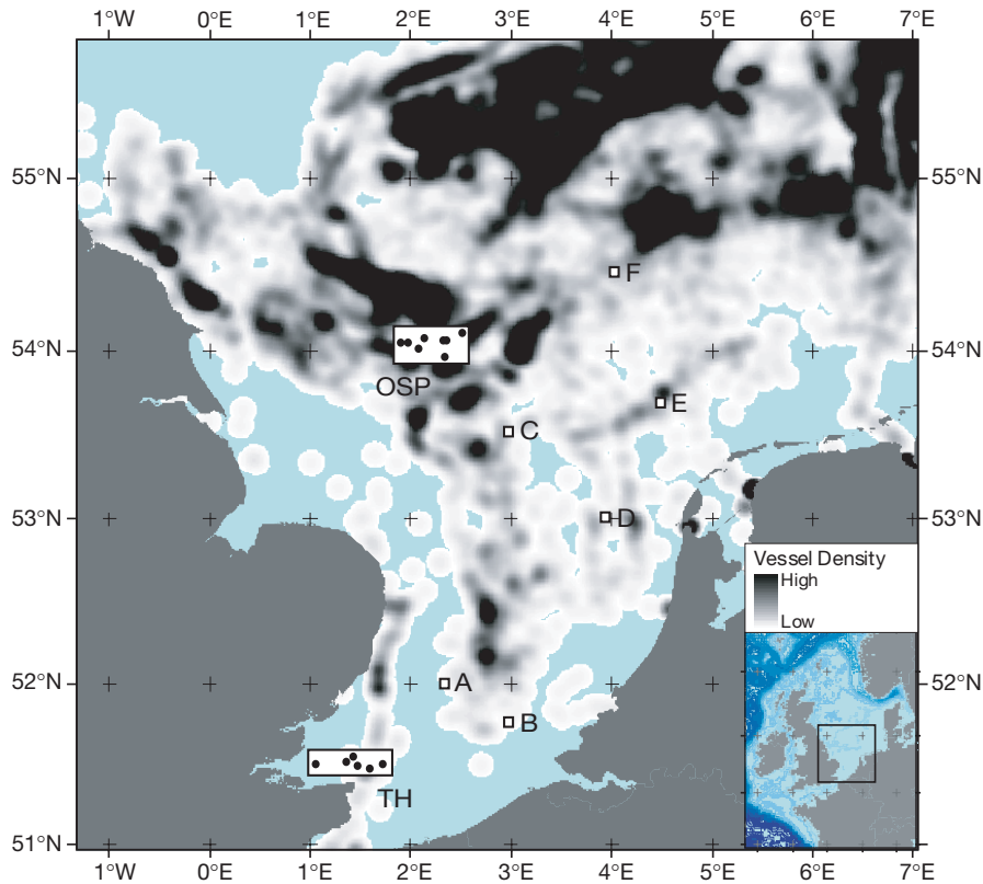
Fig. 1. Sampling sites in present study (TH: Thames; OSP: Outer Silver Pit) and other sites in the southern North Sea where biogeochemical processes have been previously measured. A: Site 12 of Trimmer et al. (2000); B: Site 1 of Upton et al. (1993); C: Site 6 of Upton et al. (1993); D: Broad Fourteens site of van Raaphorst et al. (1992) and Osinga et al. (1996); E: Frisian Front site of van Raaphorst et al. (1992); F: Oyster Grounds site of Lohse et al. (1996) and Osinga et al. (1996). Density (vessels km -2 ) of benthic trawlers operating in a portion of the southern North Sea in 2002 is also shown
