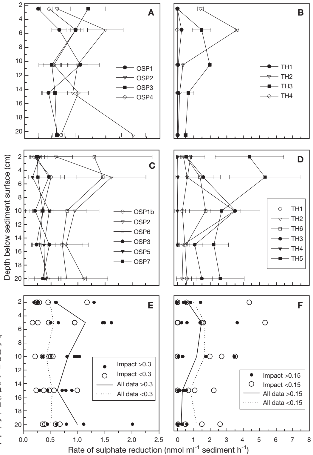
Fig. 5. Depth profiles for sulphate reduction in the OSP (left-hand graphs) and Thames (right-hand graphs) in October 2001 (A, B) and July 2002 (C, D) (means \pm SE, n = 3 ); (E, F) Mean values at each depth (both months combined) and overall mean (lines) for all replicates either side of the median impact (OSP = 0.3 SPUE, Thames = 0.15 SPUE; see 3rd sub-section of 'Results')
