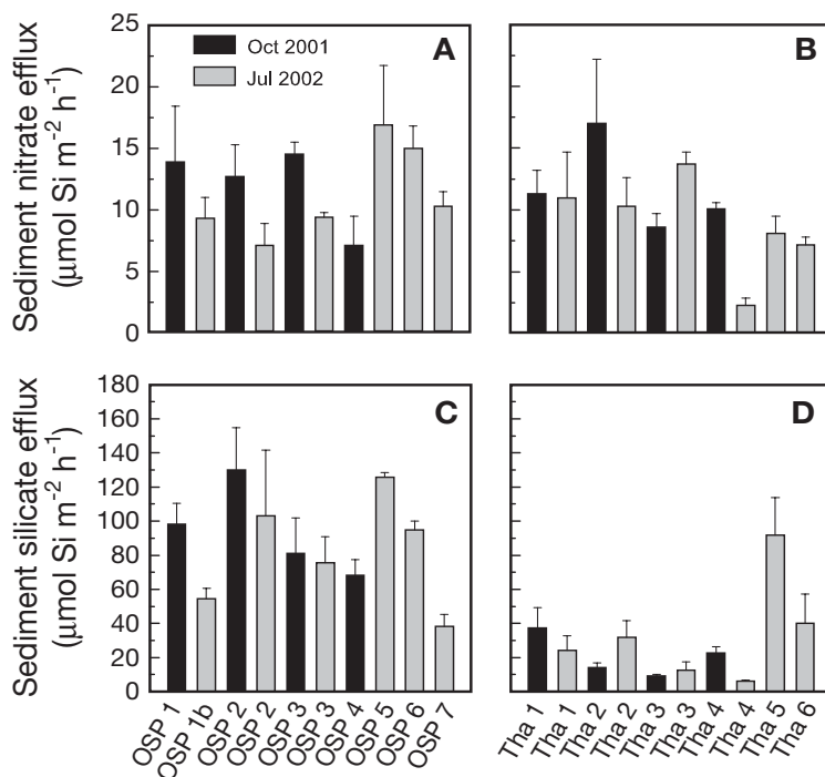
Fig. 7. Mean + SE ( n = 3 ) sediment–water nutrient exchange in OSP (left-hand graphs) and Thames (right-hand graphs) (A, B) nitrate; (C, D) silicate
