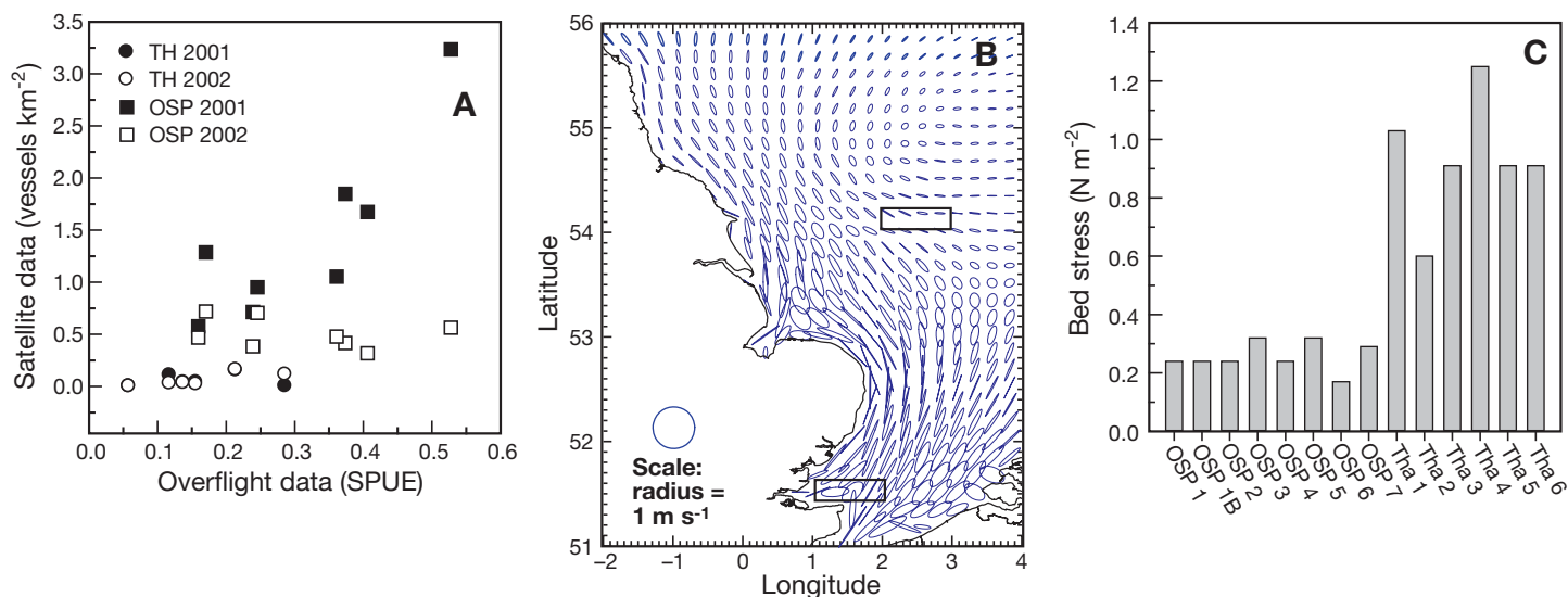
Fig. 2. Trawling impact and the tidal current data used to model bed-stress. (A) Satellite data for 2001 and 2002 plotted against long-term overflight data (1992 to 2002); SPUE: sightings per unit effort. (B) Ellipse currents and direction predicted for mean tides; the radius of scale circle corresponds to a constant speed of 1 \text{ m s}^{-1} ; upper and lower rectangles; OSP and Thames regions, respectively. (C) Model output of bed-stress ( \text{N m}^{-2} ) data at each site
