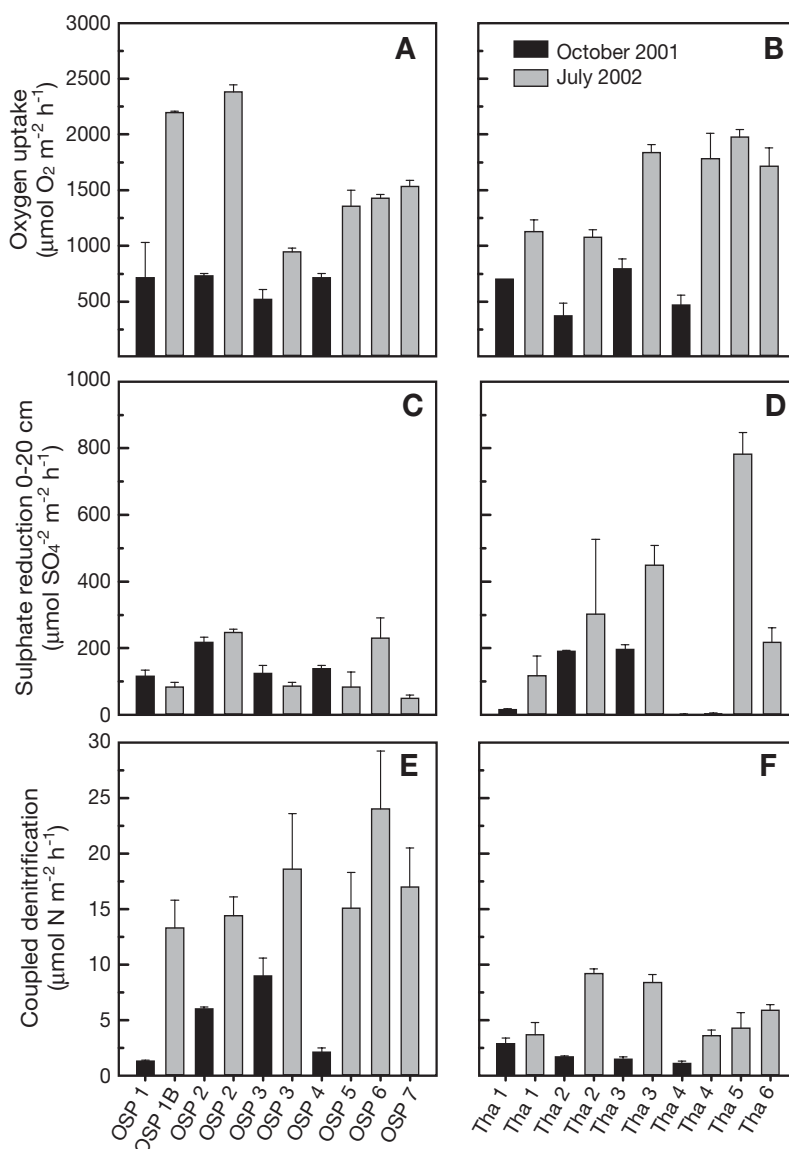
Fig. 4. Mean + SE biogeochemical process measurements for each site in October 2001 and July 2002 for OSP (A, C, E) and the Thames (B, D, F). n = 3 (except oxygen uptake at Site TH1 in October 2001, where n = 2 )
