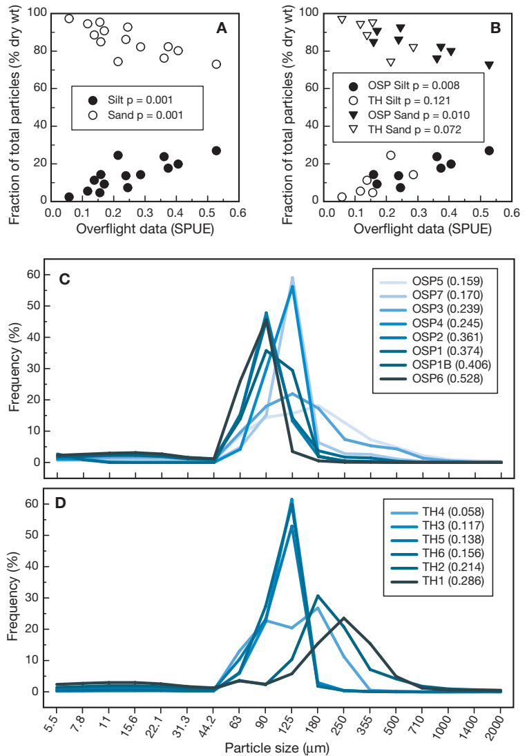
Fig. 3. Sediment grain size analysis. Average fraction of silt and sand particles as a function of SPUE for (A) all sites across both regions and (B) each region separately ( p = significance of the correlation coefficient, r ), and sediment grain size frequency distributions for each trawling impact (SPUE) in (C) OSP and (D) Thames (colour shows increasing impact from light blue to black)
