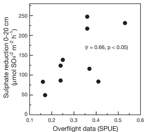
Fig. 6. Scatter-plot of areal rates of sulphate reduction against long-term overflight trawling data (SPUE) for the OSP
