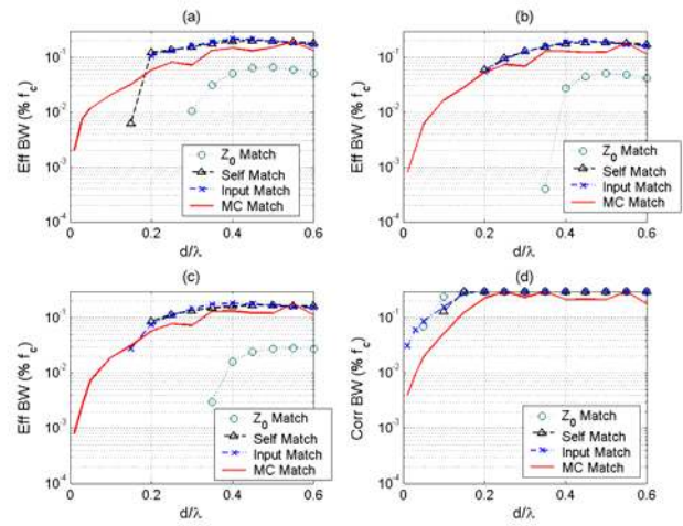
Fig. 12. Efficiency bandwidths for (a) definition (17), (b) transmit mode of Fig. 9, (c) receive mode; and (d) correlation bandwidth in receive mode of Fig. 6, over different antenna separations for different matching conditions.
