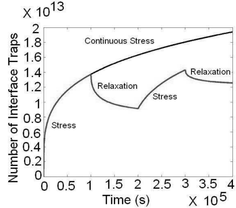
Fig. 4. N_{IT} versus t for two cycles of periodic stress and relaxation with t_0 = 10^5 seconds against the case where there is continuous stress.
