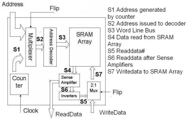
Fig. 7. Hardware implementation showing the additional hardware and control signals needed in existing SRAM arrays for periodic cell flipping
