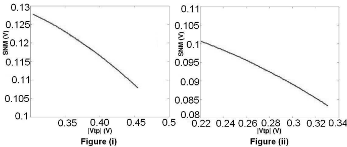
Fig. 3. SNM versus |V_{tp}| for a SRAM cell simulated at V_{dd}=1.0 V and T = 110^\circ C using (i)100nm and (ii)70nm BPTM technology.
