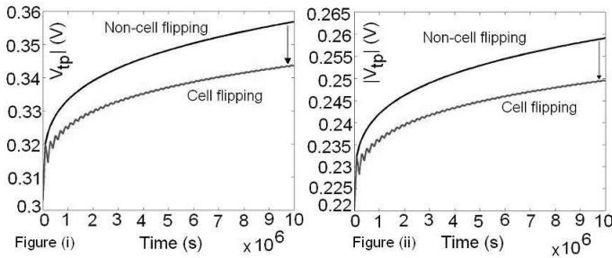
Fig. 5. |V_{tp}| versus t for periodic stress and relaxation with t_0 = 10^5 seconds for (i) 100nm and (ii) 70nm SRAM cell.
