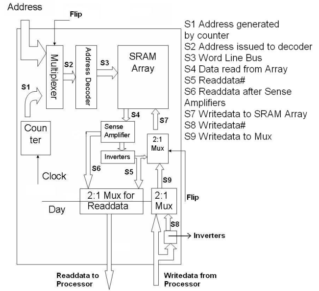
Fig. 8. Hardware implementation to ensure correct data read and write in cell flipping caches
