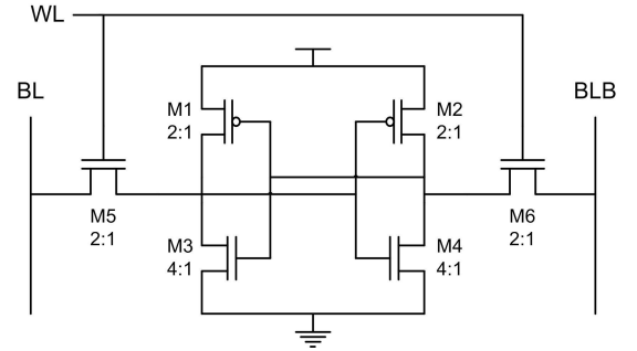
Fig. 2. Six transistor SRAM cell
