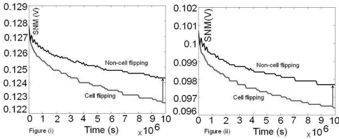
Fig. 6. SNM versus time for cell flipping and non-cell flipping case for (i) 100nm and (ii) 70nm cell.
