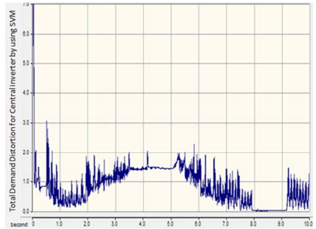
Figure 16. TDD % of the current at PCC of central using SVM.
