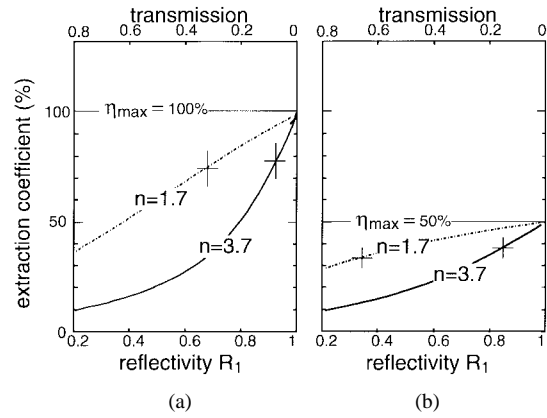
Fig. 5. (a) Extraction as a function of top mirror reflectivity R_1 for indices n = 1.7 (dash-dotted lines) and n = 3.7 (solid lines) for cavity order 1. (b) The same for cavity order 2; crosses are drawn at R_1 = 1 - m_c/n^2 .
