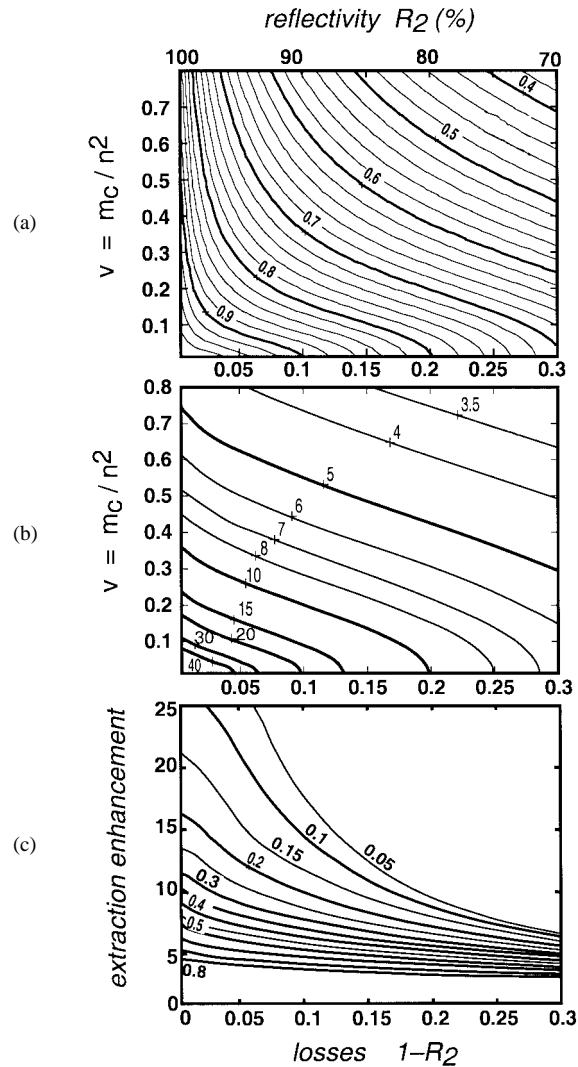
Fig. 12. (a) Optimized top mirror reflectivities R_1 contours in the (1 - R_2, v = m_c/n^2) plane. (b) Optimized extraction enhancement ( \eta/\eta_{\text{bare}} ) contours in the same plane. (c) Extraction enhancement as a function of losses, for various values of parameter v = m_c/n^2 . This is obtained from the results of (b) but can be transformed to the exact extraction of any particular case just by vertical rescaling.
