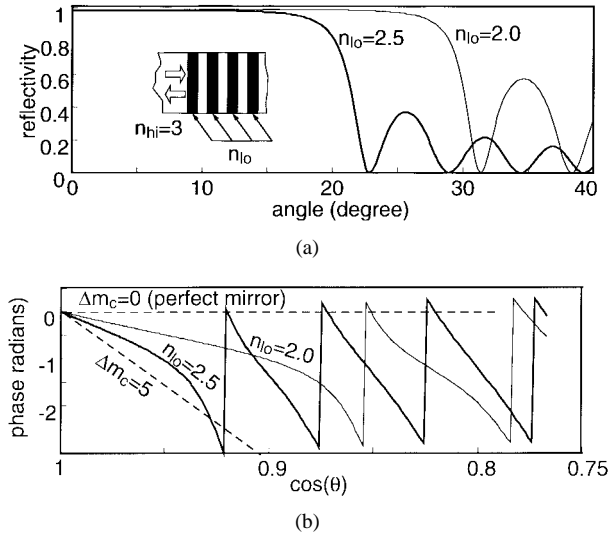
Fig. 9. (a) Power reflectivity of a DBR mirror with indices n_{hi} = 3 and n_{lo} = 2.5 or n_{lo} = 2 as a function of the angle of incidence \theta . (b) Phase of the reflectivity referenced at the first DBR layer (solid line) as a function of \cos \theta showing the linear phase shift. Dashed lines: phase of a perfect mirror located at \Delta m_c half-wavelengths for \Delta m_c = 0 and 5.
