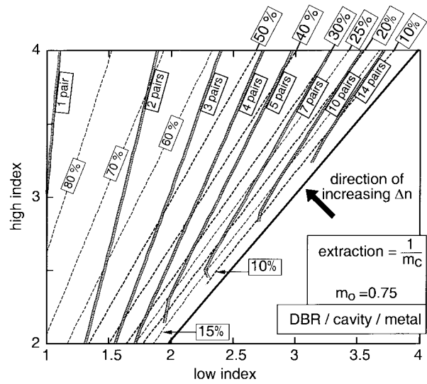
Fig. 11. Contour map of approximate extraction efficiency \eta (thinner dashed lines) and critical number of DBR pairs [according to (28), thicker lines] in the (n_{\text{lo}}, n_{\text{hi}}) plane for an asymmetric DBR/cavity/metal light-emitting structure: the source is monochromatic, the metal is lossless, the antinode factor is \zeta = 1 , and the bare cavity order is m_o = 0.75 (see Fig. 3 of [Section II] for comparison). The index contrast \Delta n increases linearly above the n_{\text{lo}} = n_{\text{hi}} line. Validity tends to break down for large \Delta n and \eta > 50\% .
