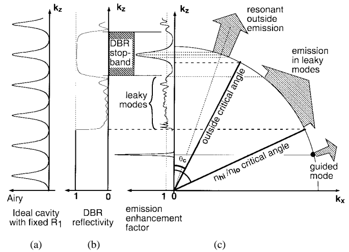
Fig. 13. Same plot as Figs. 3 and 4 when using DBR mirrors. (a) Comb-like Airy function of an ideal cavity with constant reflectivities. (b) DBR reflectivity, with the stopband, the window at smaller k_z and the about total reflection at critical angle with the low index medium. (c) Modified Airy function, with the extracted FP peak, but losing the structure of (a) especially in the leaky mode region. Emission in the various modes is indicated.
