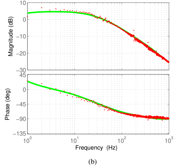
Fig. 12: Frequency response of the impedance: (a) the impedance of the current source subsystem and (b) the impedance of the voltage source subsystem (solid-line is from model prediction and the red-points are from detailed simulation).
