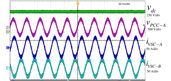
Fig. 7: Experimental results for -10 kW power reference to the VSC-A (Stable case): (i) the dc link voltage, (ii) voltage at PCC of VSC (phase-A), (iii) current of VSC-A (phase-A) and (iv) current of VSC-B (phase-A).
