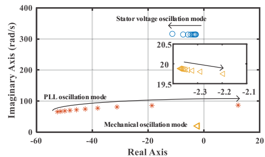
Fig. 8. Dominated eigenvalues of the grid connected DFIG with the increase of the PLL parameters
