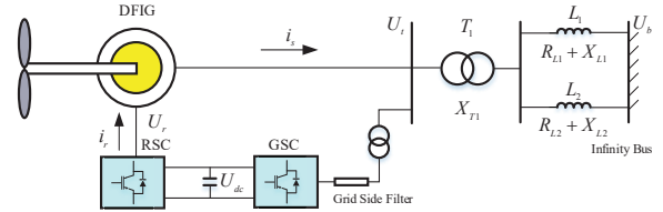
Fig. 2. Single grid-connected DFIG wind farm
