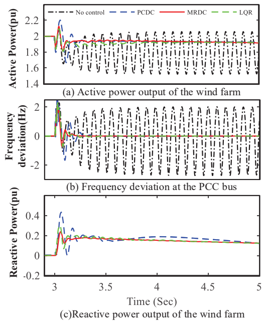
Fig. 18. Response of power output of wind farm and frequency deviation the system under the S_{rip} = 1.20
