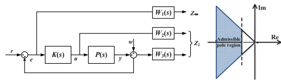
Fig. 15. Block diagram of the mixed H_2/H_\infty robust damping controller
