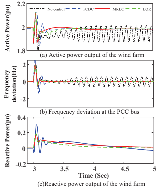
Fig. 17. Response of power output of wind farm and frequency deviation the system under the S_{tip} = 1.38
