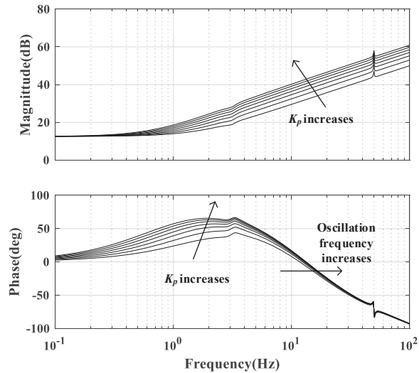
Fig. 13. Bode diagram of the control loop including PLL under different K_P
