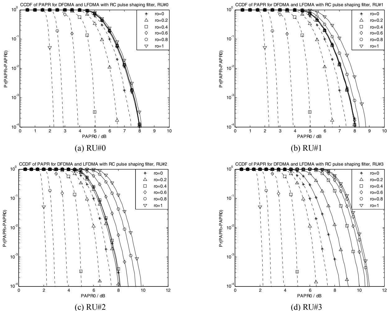
Fig. 3: CCDF of PAPR for DFDMA (dashed line) and LFDMA (solid line) signals using raised cosine (RC) pulse shaping filter with \alpha = 0, 0.2, 0.4, 0.6, 0.8 and 1 . * r_0 = rolloff factor, \alpha .
