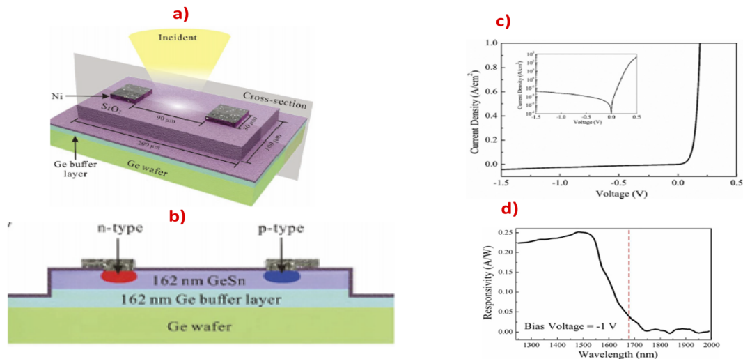
Fig. 50 (a) Structure of GeSn/i-GeSn on Ge wafer devices, (b) cross section of the device, (c) effect of applied voltage on the current density, and (d) responsivity of the diode at a bias voltage of -1 V. "Reproduced from ref. 168 with permission from [American Institute of Physics publisher], copyright [2020]".
