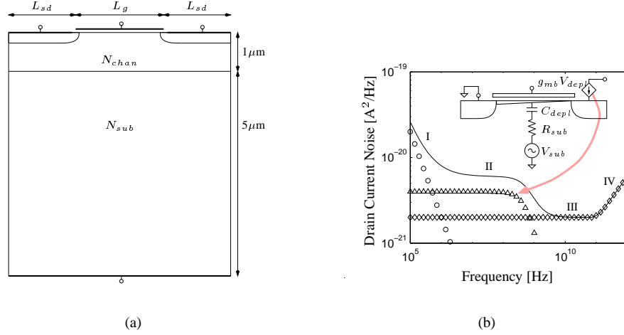
Fig. 1. (a) Cross-section of the MOSFET structure used for simulation. (b) Anticipated general drain current noise power spectrum for bulk MOSFETs. The solid line is total noise power, the circle symbol is the 1/f noise component ( S_{i_d,1/f} ), the triangle symbol is the additive component induced by the substrate ( S_{i_d,sub} ), and the diamond symbol is the channel thermal noise component ( S_{i_d,channel} ). The inset circuit diagram explains the contribution mechanism of the substrate thermal noise to the drain current noise.
