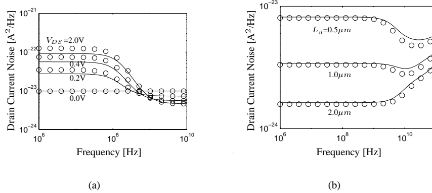
Fig. 2. Simulation results of drain current noise power spectrum. The gate oxide thickness is 60nm, N_{chan} is 5.0 \times 10^{17} \text{cm}^{-3} , L_{sd} is 0.01 \mu\text{m} , and V_{GS} is 1.5V. The symbols are PADRE simulation results and lines are calculated using (2). (a) A 0.5 \mu\text{m} MOSFET for different drain bias conditions. N_{sub} is 1.0 \times 10^{15} \text{cm}^{-3} . (b) MOSFETs with different gate lengths. N_{sub} is 3.2 \times 10^{16} \text{cm}^{-3} , and V_{DS} is 2.5V.
