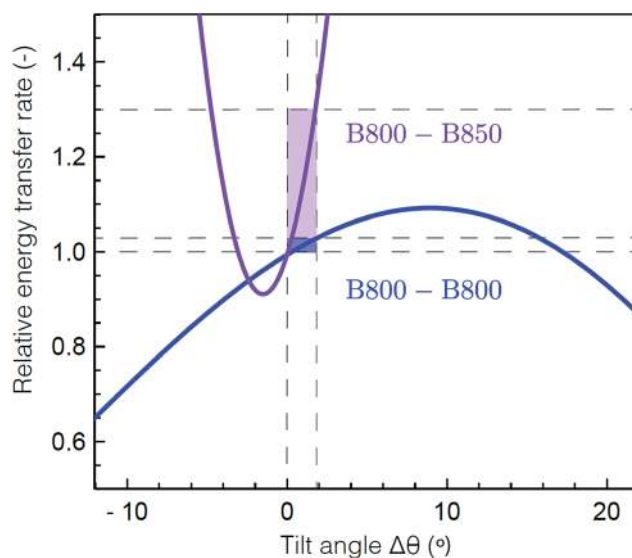
Fig. 4 Theoretical energy transfer rates within LH2. The energy transfer rates within B800 (blue) and between B800 and B850 (purple) as a function of a tilt in the orientation of the B800 transition dipole moments relative to the original structure. 59 A positive tilt results in a steady increase of the B800 rate from the original geometry, up to a maximum obtained for a tilt of \Delta\theta = 9^\circ corresponding to a flat B800 ring. The shaded domains illustrate the range for which the B800 rate increases by 1% (blue) and the corresponding, drastic change in the inter-ring transfer rate (purple). Flattening the B800 BChls by 2^\circ enhances the B800–B850 rate by more than 30%. The presented B800–B850 rate displays the average rate from one B800 BChl to the six nearest B850 BChls.
