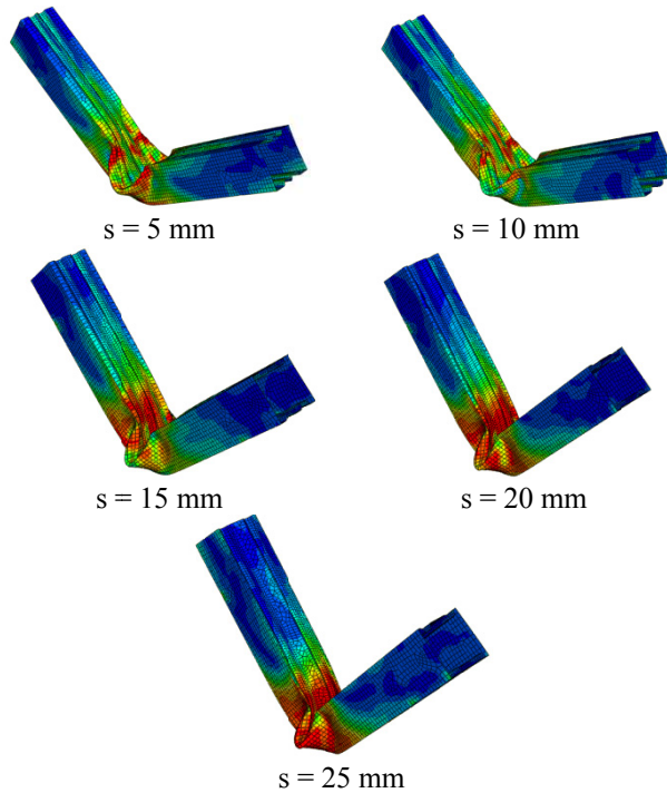
Figure 25. Deformed shapes of 2-grooved SHS column with impact speed of 14 m/s and impact mass of 5 kg
