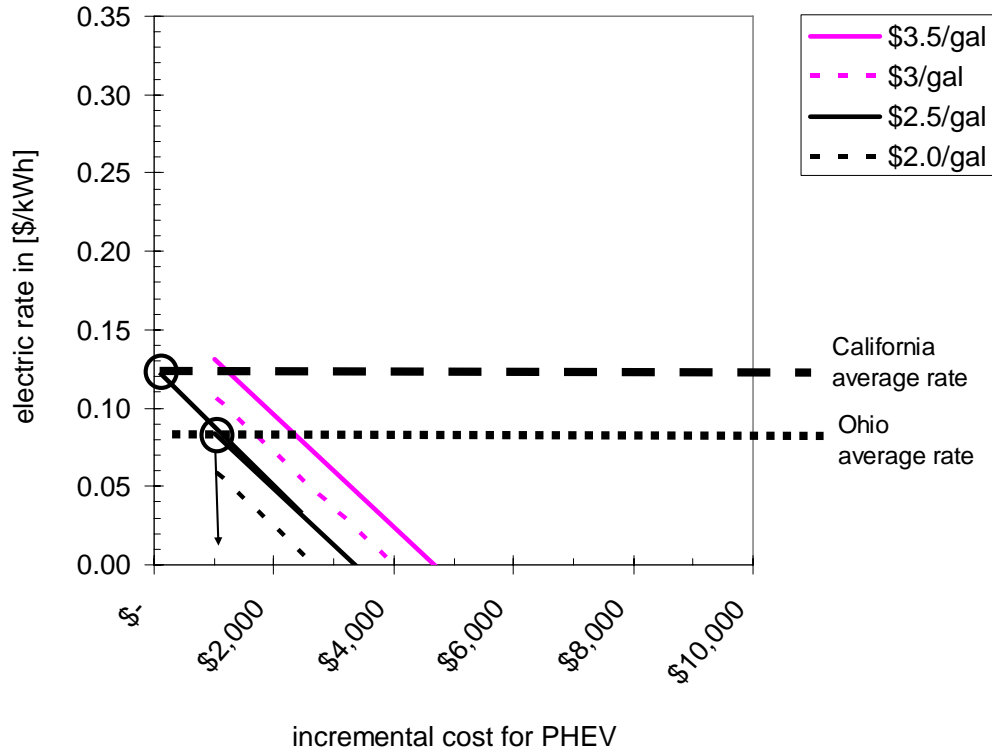
Figure 3: Results of The Life-Cycle Cost Analysis for a PHEV Compared with a Toyota Prius with 56 MPG Mixed City-Highway Fuel Economy. Diagonal Lines Denote the Break-Even Point.
