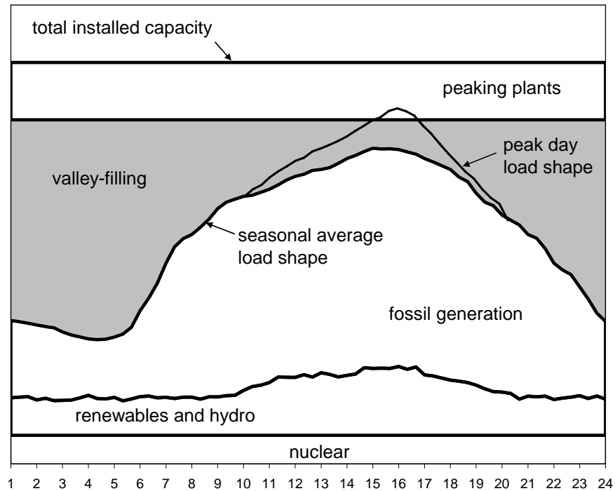
Figure 2: Stylized Load Shape for 1 Day During Peak Season, Generation Dispatch, and Installed Capacity
