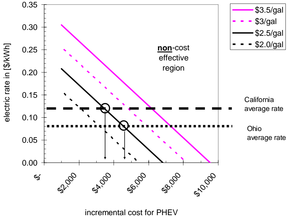
Figure 2: Results of the Life-Cycle Cost Analysis for a PHEV Compared with a Conventional Vehicle with 27.5 MPG Fuel Economy. Diagonal Lines Denote the Break-Even Point.
