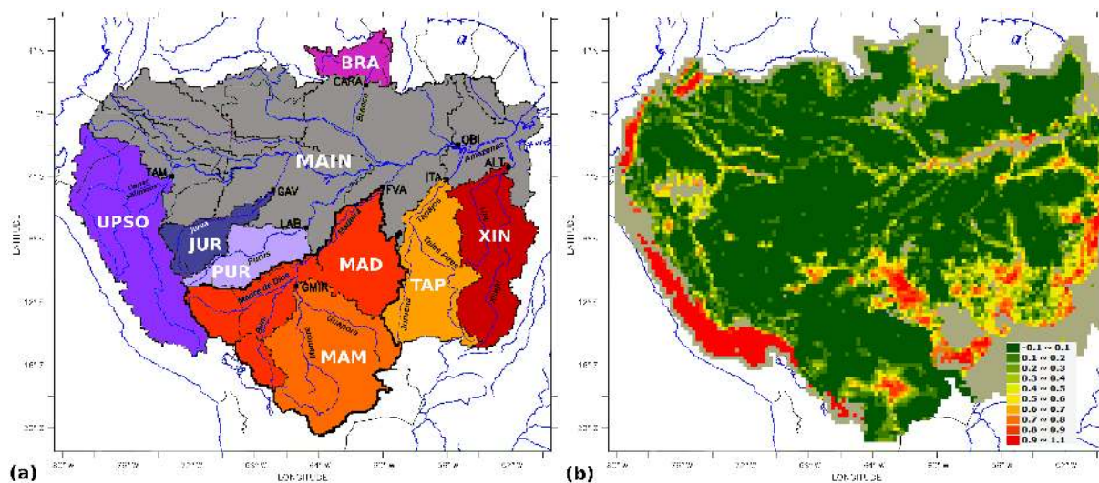
Figure 1. Panel (a) indicates Amazon catchments (names in white; the abbreviations are indicated in Table S1) and the main rivers (adapted from Guimberteau et al., 2012), with localization of the main SO HYBAM gauging stations (the abbreviations are indicated in Table S1). The bold black line delineates the Madeira catchment. Colour is used to distinguish the southern (red), western (purple) and northern catchments (pink). Panel (b) indicates the percentage of deforestation in each 25 \times 25 \text{ km}^2 in 2005 (observed data; Aguiar et al., 2016).
