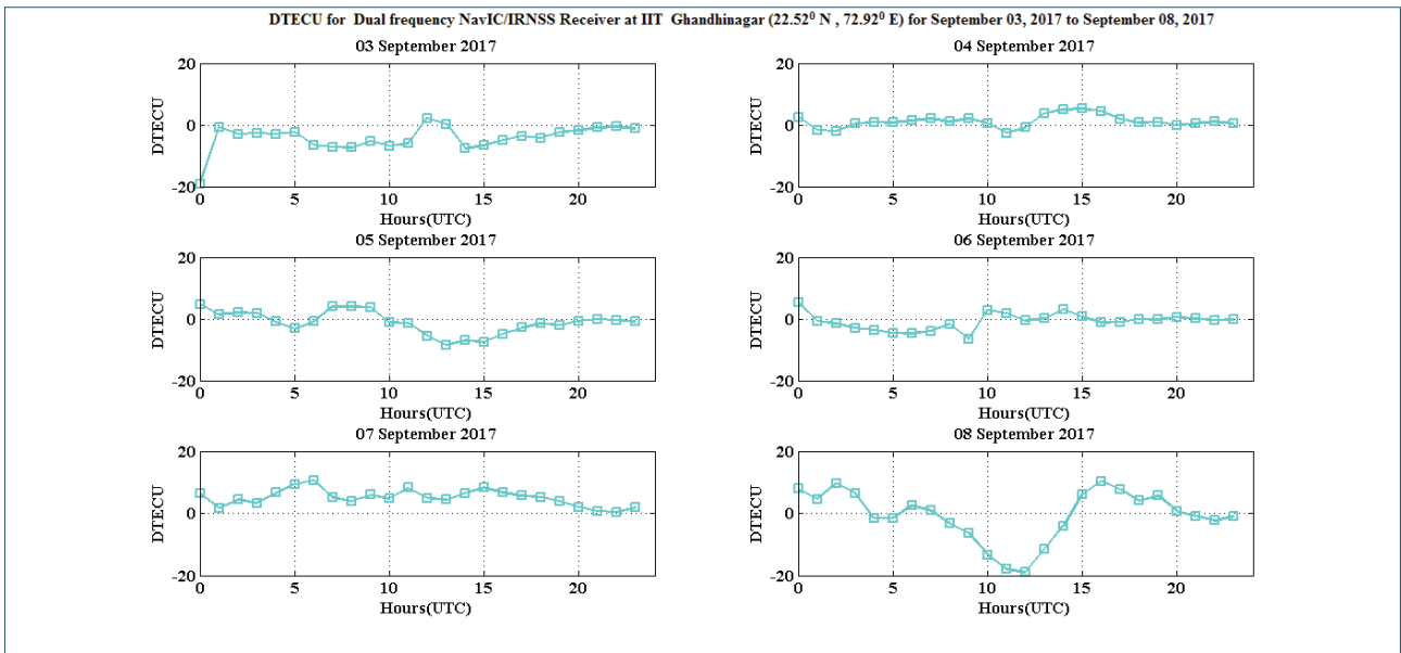
FIGURE 13. DTECU for Dual frequency NavIC/IRNSS Receiver at IIT Gandhinagar (22.52° N latitude, 72.92° E Longitude) for September 03, 2017 to September 08, 2017
