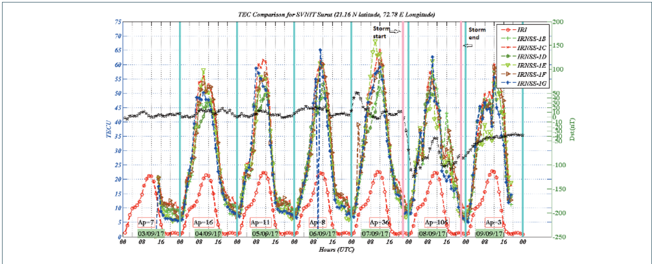
FIGURE 4. TEC Comparison between IRI-Model and Dual frequency NavIC/IRNSS Receiver for SVNIT Surat (21.16° N latitude, 72.78° E Longitude).
