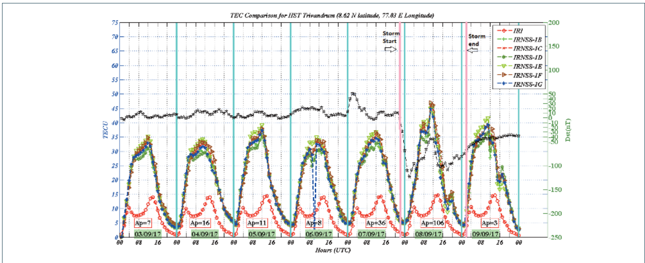
FIGURE 8. TEC Comparison between IRI-Model and Dual frequency NavIC/IRNSS Receiver for IIST Trivandrum (8.62° N latitude, 77.03° E Longitude).
