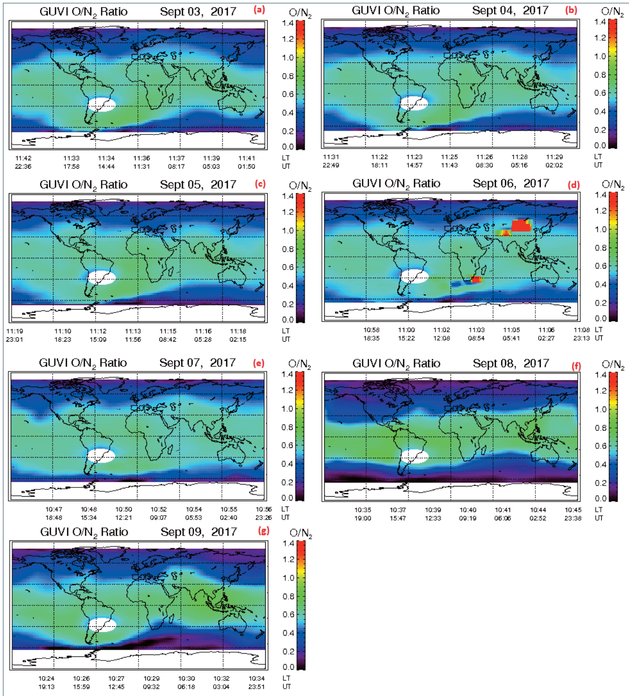
FIGURE 14. Global Thermospheric O/N_2 Mapping using GUVI data server.
