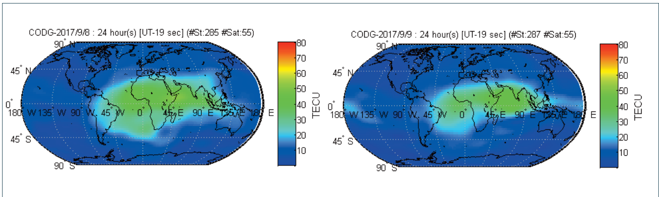
FIGURE 15. (d) Global TEC Mapping (Two hours resolution) comparison (8 September 2017 and 9 September 2017) using global IONEX file from GNSS IGS data server ( 24 hours).
