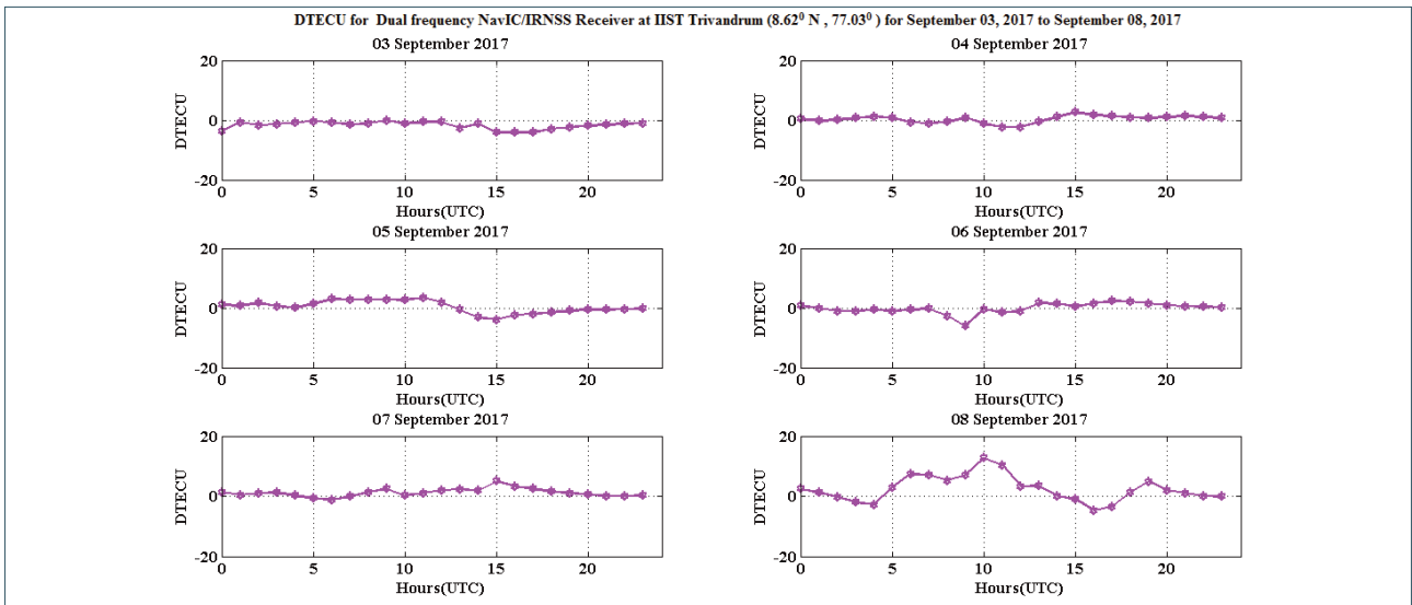
FIGURE 9. DTECU for Dual frequency NavIC/IRNSS Receiver at IIST Trivandrum (8.62° N latitude, 77.03° E Longitude) for September 03, 2017 to September 08, 2017.
