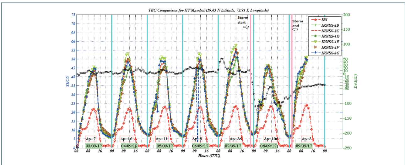
FIGURE 5. TEC Comparison between IRI-Model and Dual frequency NavIC/IRNSS Receiver for IIT Mumbai (19.03° N latitude, 72.91° E Longitude).
