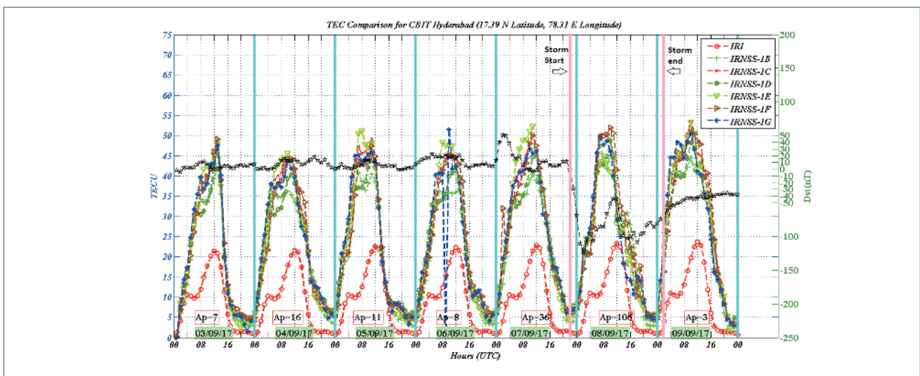
FIGURE 6. TEC Comparison between IRI-Model and Dual frequency NavIC/IRNSS Receiver for CBIT Hyderabad (17.39° N latitude, 78.31° E Longitude)
