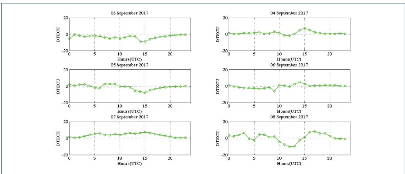
FIGURE 11. DTECU for Dual frequency NavIC/IRNSS Receiver at IIT Mumbai (19.03° N latitude, 72.91° E Longitude) for September 03, 2017 to September 08, 2017.
