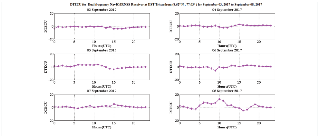
FIGURE 10. DTECU for Dual frequency NavIC/IRNSS Receiver at CBIT Hyderabad (17.39° N latitude, 78.31° E Longitude) for September 03, 2017 to September 08, 2017.
