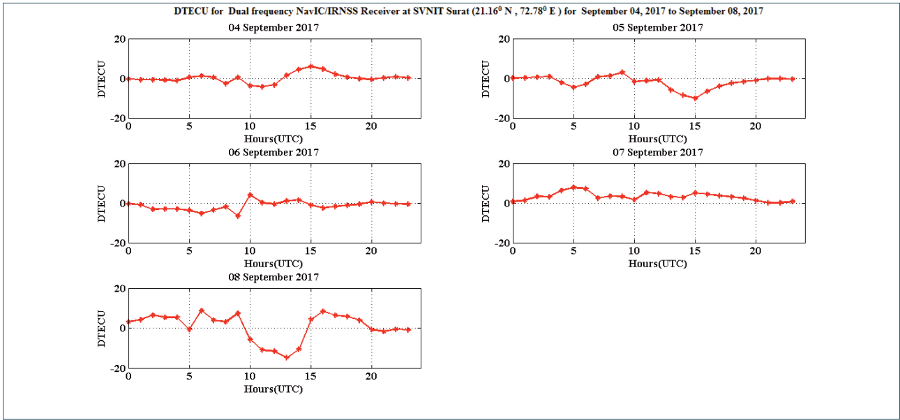
FIGURE 12. DTECU for Dual frequency NavIC/IRNSS Receiver at SVNIT Surat (21.16° N latitude, 72.78° E Longitude) for September 04, 2017 to September 08, 2017
