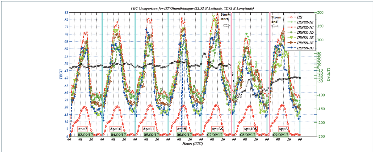
FIGURE 7. TEC Comparison between IRI-Model and Dual frequency NavIC/IRNSS Receiver for IIT Gandhinagar (22.52° N latitude, 72.92° E Longitude).
