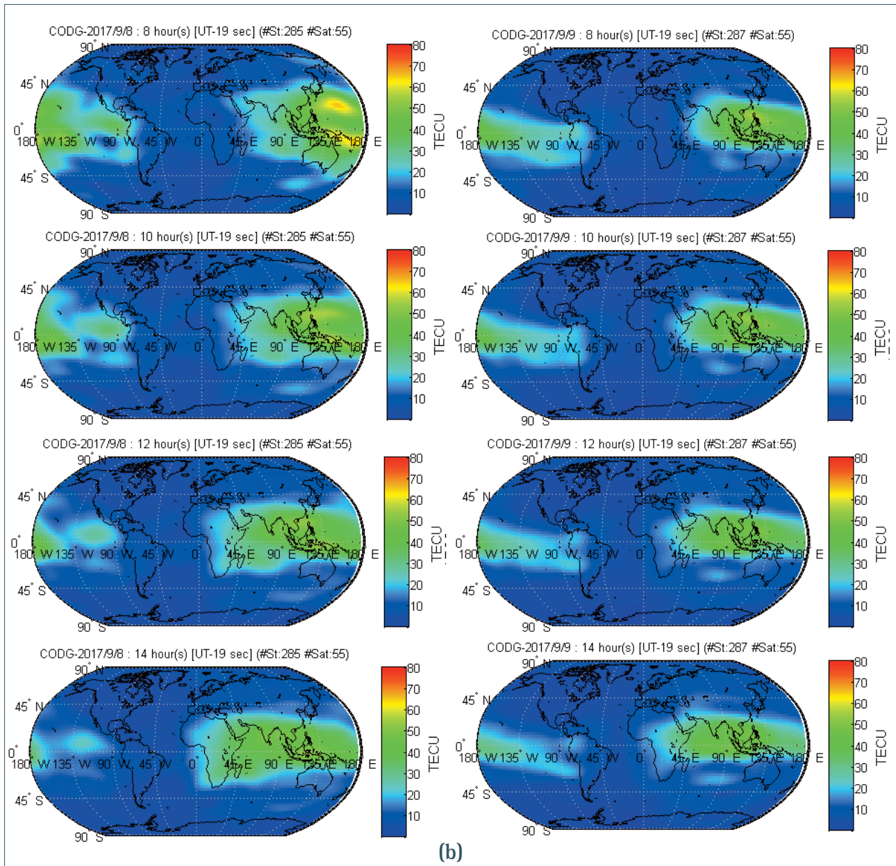
FIGURE 15. (b) Global TEC Mapping (Two hours resolution) comparison (8 September 2017 and 9 September 2017) using global IONEX file from GNSS IGS data server (08-14 hours).
