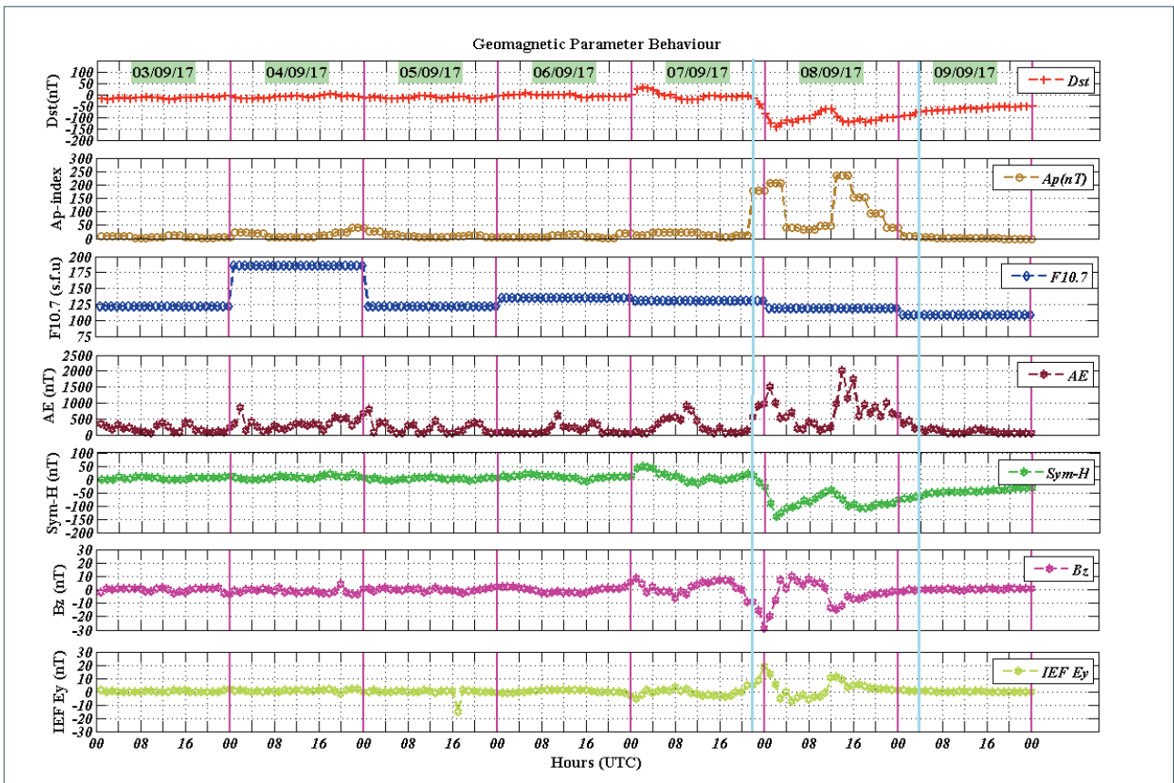
FIGURE 2. Graphical Representation of various geomagnetic parameters.
