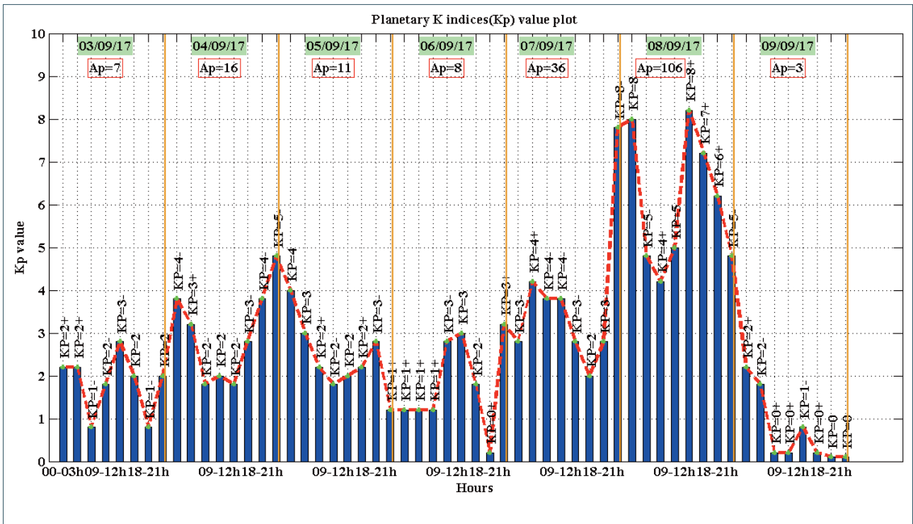
FIGURE 1. Graphical Representation of Kp Indices.
