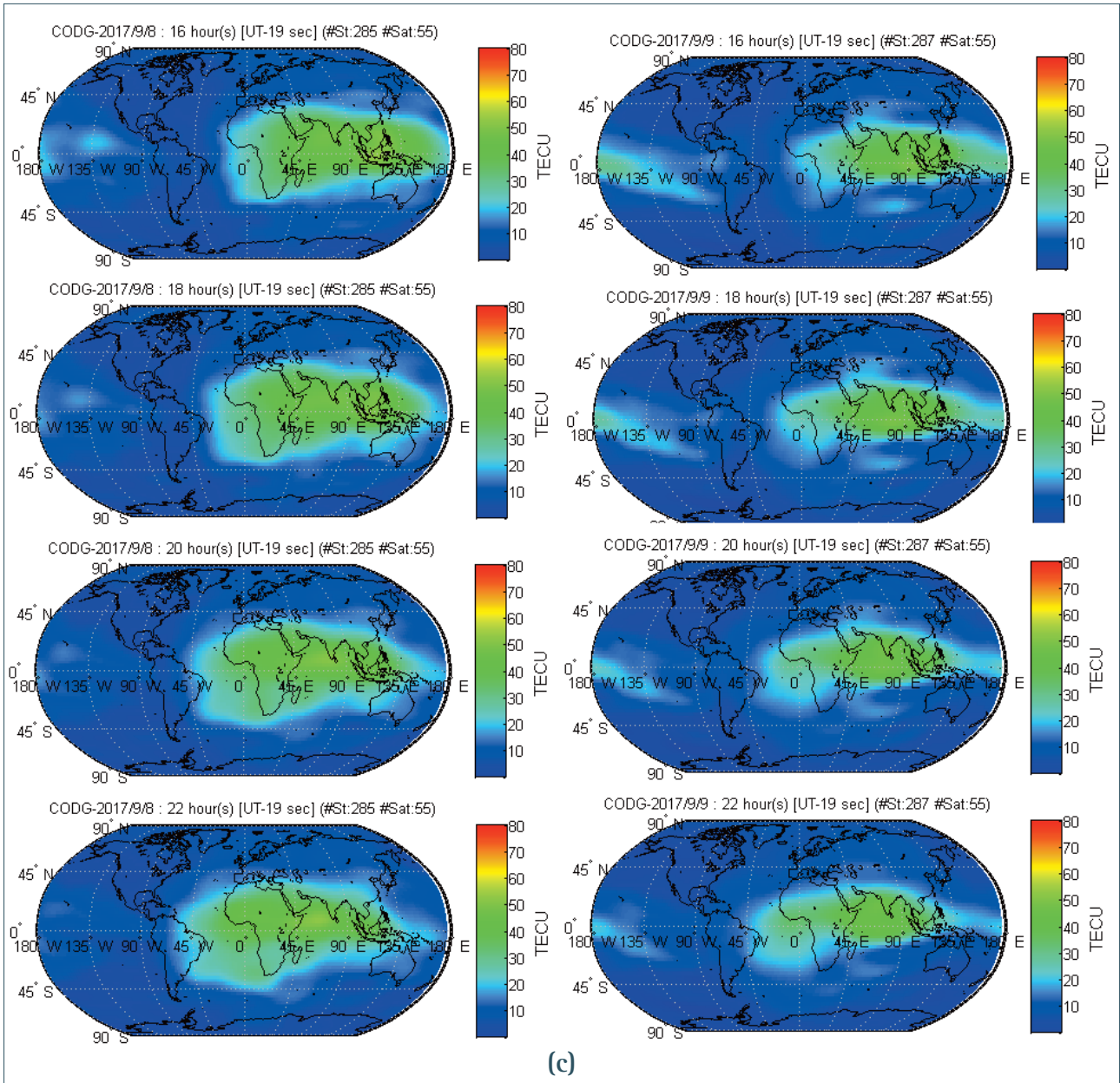
FIGURE 15. (c) Global TEC Mapping (Two hours resolution) comparison (8 September 2017 and 9 September 2017) using global IONEX file from GNSS IGS data server ( 16-22hours).
