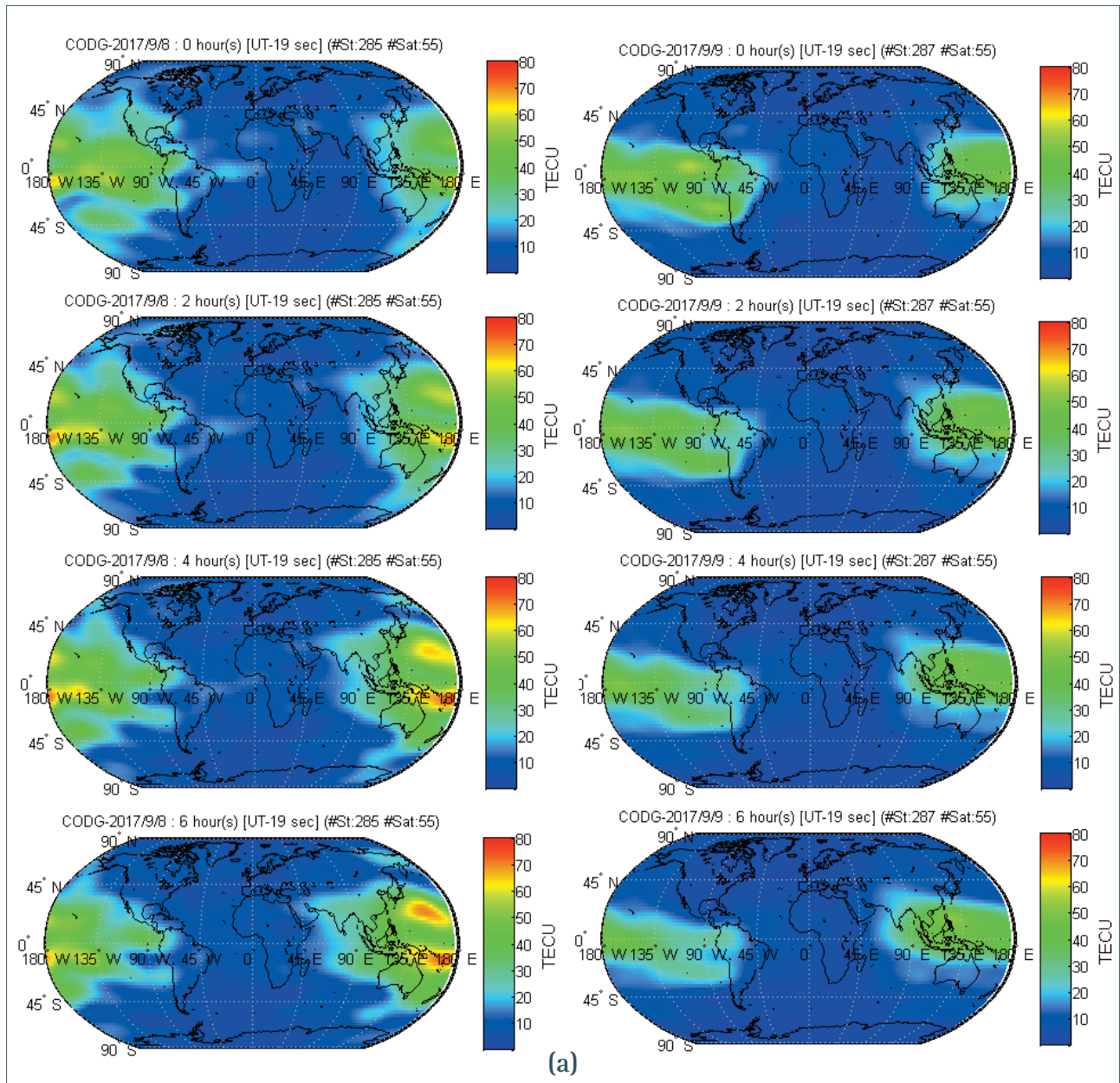
FIGURE 15. (a) Global TEC Mapping (Two hours resolution) comparison (8 September 2017 and 9 September 2017) using global IONEX file from GNSS IGS data server (00-06 hours).
