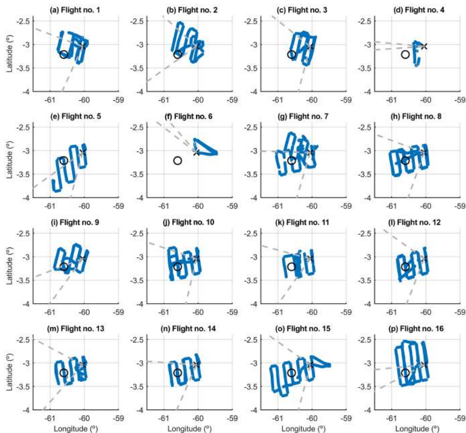
Figure 2. Trajectories for all G-1 flights during GoAmazon2014/5 IOP1. Manaus is located close to the \{-60, -3\} point, marked with an “X”, while the T3 site is marked with the black circle.
