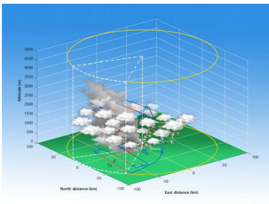
Figure 1. Conceptual schematic for the flight patterns planning. It shows Manaus city and its pollution plume dispersing over the surrounding Amazon forest. The Cu field shown is very common during the wet season and is representative for most of the cloud conditions during the flights. The yellow circles indicate a 100 km radius from Manaus airport, although the figure is not meant to be quantitatively accurate. The lines with arrow heads show the most common flight plan used, where blue regions are possible locations for the background air measurements and the red ones indicate measurements inside the plume section (dashed white lines). T3 is a GoAmazon site to the north of Manacapuru.
