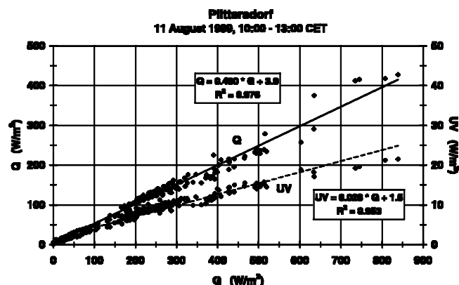
Figure 4: Relationships between global radiation G and net radiation Q as well as UV radiation UV during the solar eclipse of 11 August 1999 at the Plittersdorf site.
