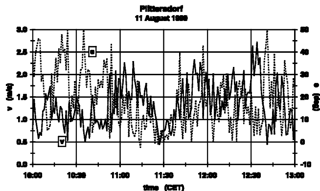
Figure 8: Horizontal wind speed v and elevation angle e of the three-dimensional wind vector at 17 m above ground level during the solar eclipse of 11 August 1999 at the Plittersdorf site.
