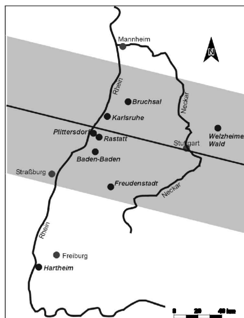
Figure 1: Mid-eclipse and zone of totality of the solar eclipse of 11 August 1999 in south-west Germany.
