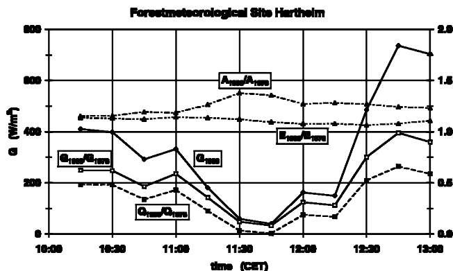
Figure 6: Global radiation G during the solar eclipse of 11 August 1999 as well as ratios of G , upward longwave radiation E , downward longwave radiation A and net radiation Q measured during the solar eclipses of 11 August 1999 and 29 April 1976 at the Forest-meteorological Site Hartheim.
