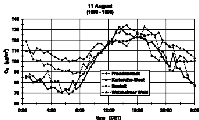
Figure 16: Half-hourly mean values of \text{O}_X (i.e. \text{O}_3 + \text{NO}_2 ) on 11 August at the official air quality stations Freudenstadt, Karlsruhe-West, Rastatt, and Welzheimer Wald averaged over the period 1989 to 1998.
