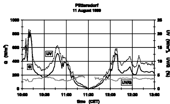
Figure 3: Global radiation G , UV radiation UV and ratio UV/G during the solar eclipse of 11 August 1999 at the Plittersdorf site.
