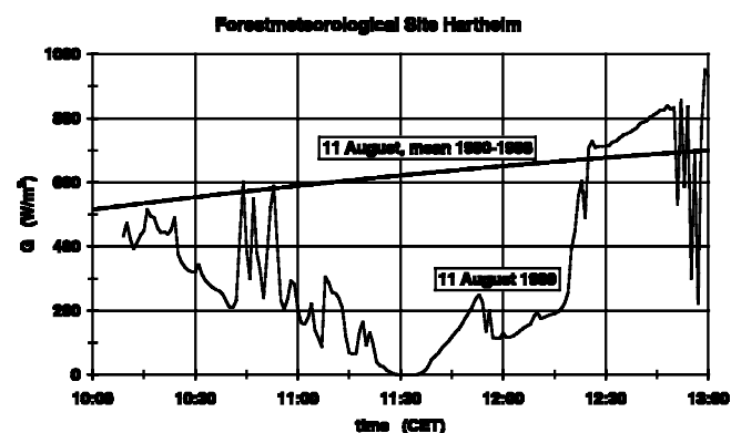
Figure 5: Global radiation G during the solar eclipse of 11 August 1999 compared with that of nine years average (1990–1998) for 11 August at the Forestmeteorological Site Hartheim.
