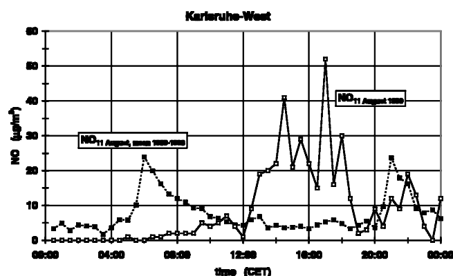
Figure 15: Half-hourly mean values of nitrogen oxide ( \text{NO} ) on 11 August 1999 compared with that of ten years average (1989–1998) measured at the official air quality station Karlsruhe-West.
