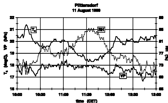
Figure 7: Air temperature T_a , vapour pressure VP and relative humidity RH at screen level during the solar eclipse of 11 August 1999 at the Plittersdorf site.
