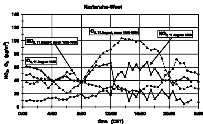
Figure 12: Half-hourly mean values of nitrogen dioxide ( \text{NO}_2 ) and ozone ( \text{O}_3 ) on 11 August 1999 compared with that of ten years average (1989–1998) measured at the official air quality station Karlsruhe-West for 11 August.
