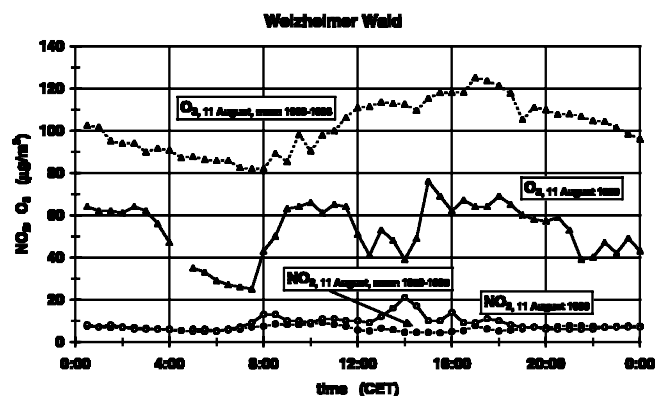
Figure 14: Half-hourly mean values of nitrogen dioxide ( \text{NO}_2 ) and ozone ( \text{O}_3 ) on 11 August 1999 compared with that of ten years average (1989–1998) measured at the official air quality station Welzheimer Wald for 11 August.
