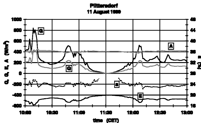
Figure 2: Global radiation G , shortwave albedo a , upward longwave radiation E , downward longwave radiation A and net radiation Q during the solar eclipse of 11 August 1999 at the Plittersdorf site.
