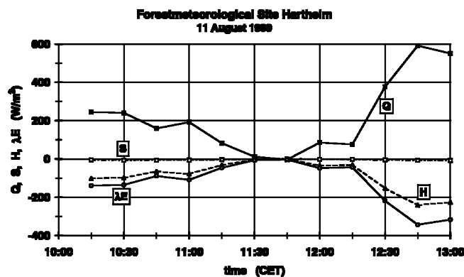
Figure 10: 15 minute mean values of net radiation Q , soil heat flux S , turbulent heat flux of sensible heat H and turbulent flux of latent heat \lambda E for the Scots pine stand at the Forestmeteorological Site Hartheim during the solar eclipse of 11 August 1999.
