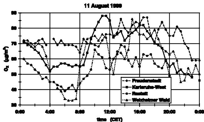
Figure 17: Half-hourly mean values of O_X (i.e. O_3 + NO_2 ) on 11 August 1999 at the official air quality stations Freudenstadt, Karlsruhe-West, Rastatt and Welzheimer Wald.
