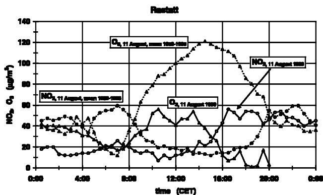
Figure 13: Half-hourly mean values of nitrogen dioxide ( \text{NO}_2 ) and ozone ( \text{O}_3 ) on 11 August 1999 compared with that of ten years average (1989–1998) measured at the official air quality station Rastatt for 11 August.
