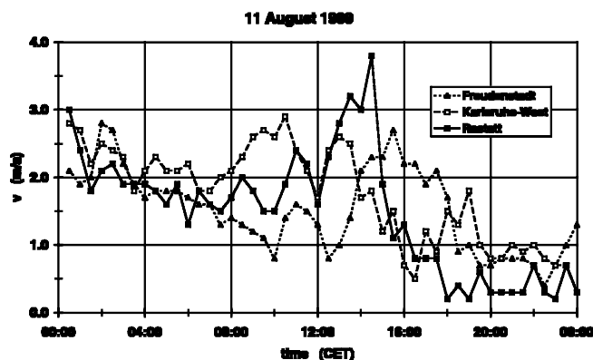
Figure 9: Half-hourly mean values of horizontal wind speed v at 10 m above ground level on 11 August 1999 at the official air quality stations Freudenstadt, Karlsruhe-West and Rastatt in Baden-Wuerttemberg.
