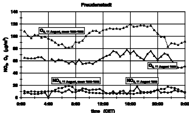
Figure 11: Half-hourly mean values of nitrogen dioxide ( \text{NO}_2 ) and ozone ( \text{O}_3 ) on 11 August 1999 compared with that of ten years average (1989–1998) measured at the official air quality station Freudenstadt for 11 August.
