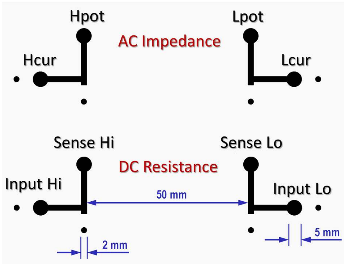
Figure 1 The pre-deposited silver electrodes design and location of electrical probes
