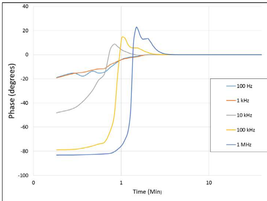
Figure 12 The phase measurement during cure at 95°C for GEM 1
