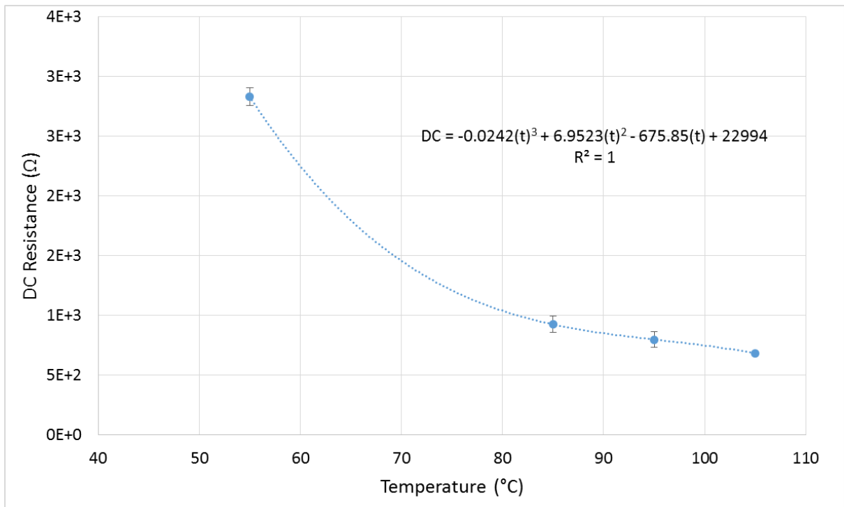
Figure 16 The DC resistance measurements of Paste E after 40 minutes at different curing temperature
