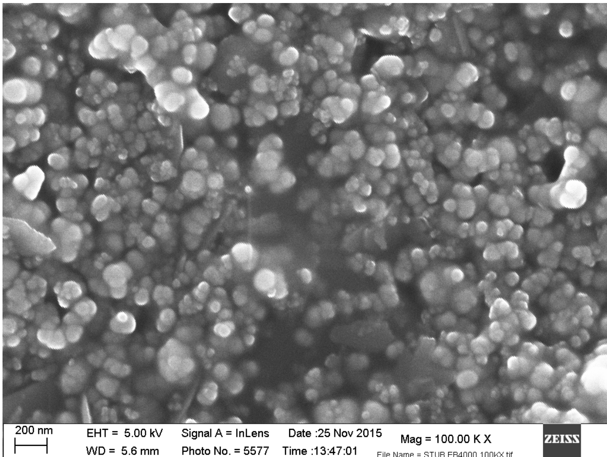
Figure 8 SEM image of Paste E
