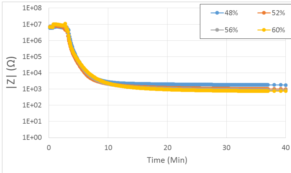
Figure 15 Impedance measurement at 1 MHz of Paste E at different particle loading
