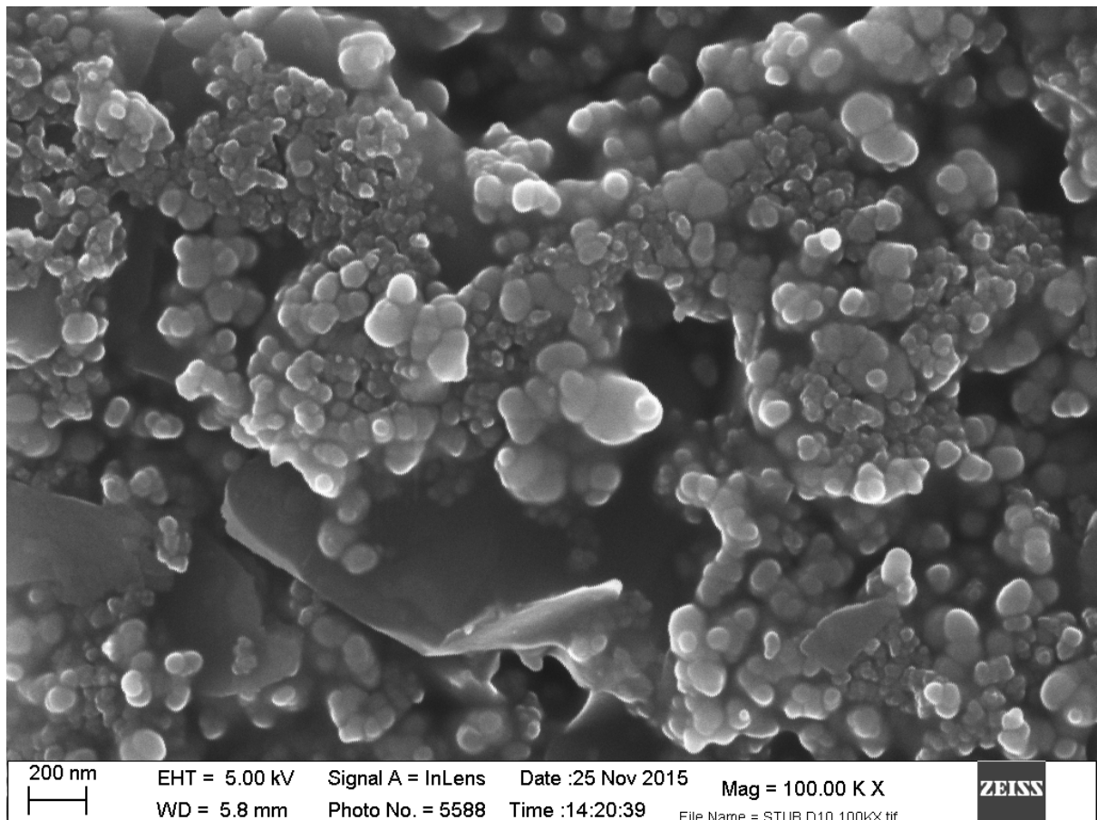
Figure 9 SEM image of GEM 1
