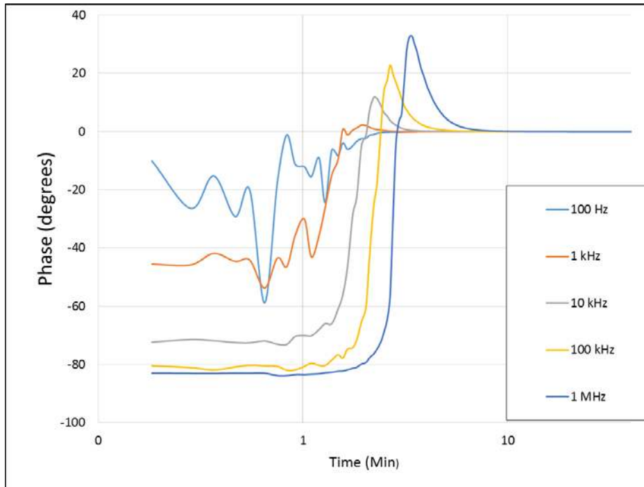
Figure 11 The phase measurement during cure at 95°C for Paste E
