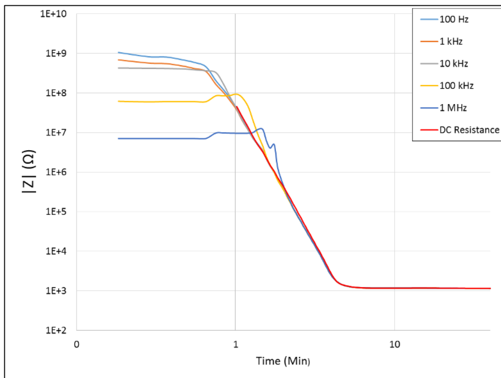
Figure 7 The AC impedance and DC resistance measurement during cure at 95°C for GEM 2
