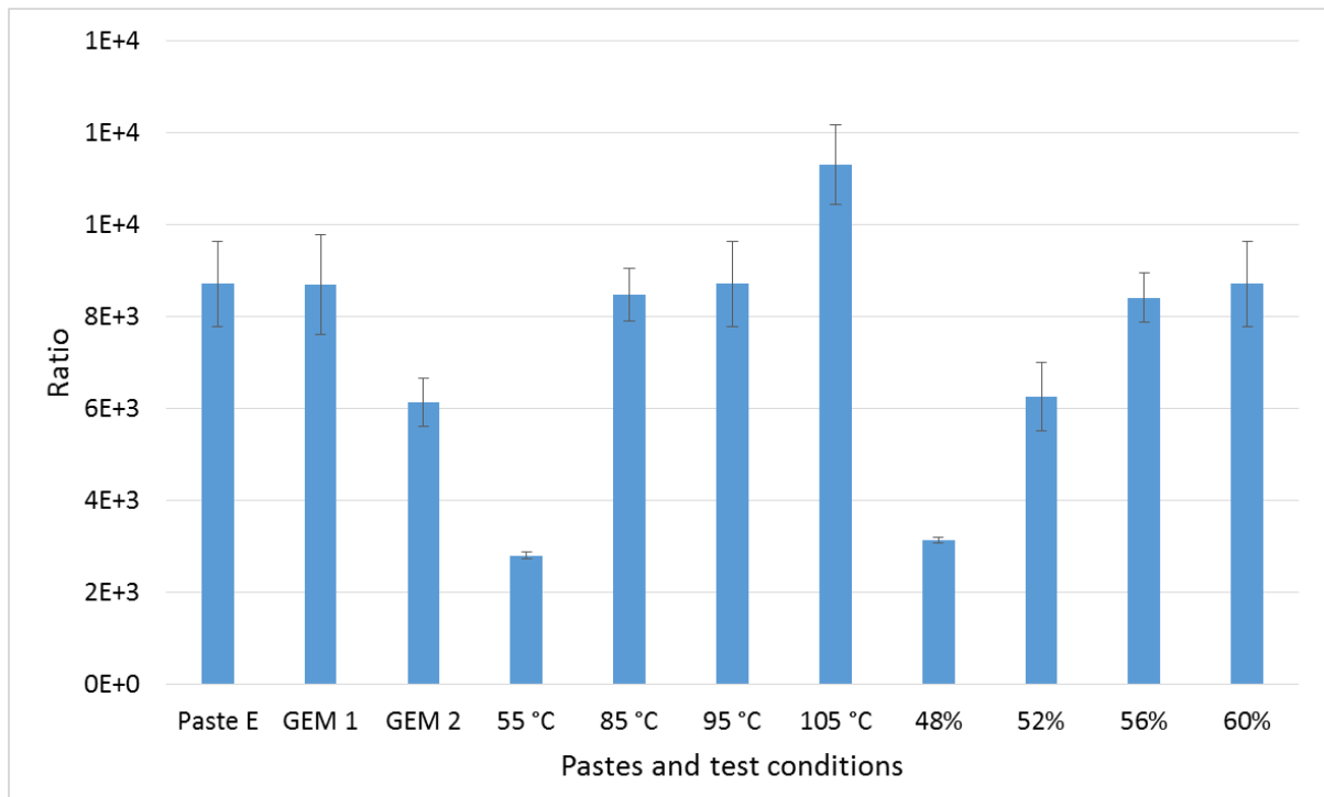
Figure 18 The AC (T0) / DC (T40) ratio of different pastes , and Paste E for various curing temperature and particle loading. The blue bars show the average values and the error bars show standard deviation for 5 measurements in each test condition
