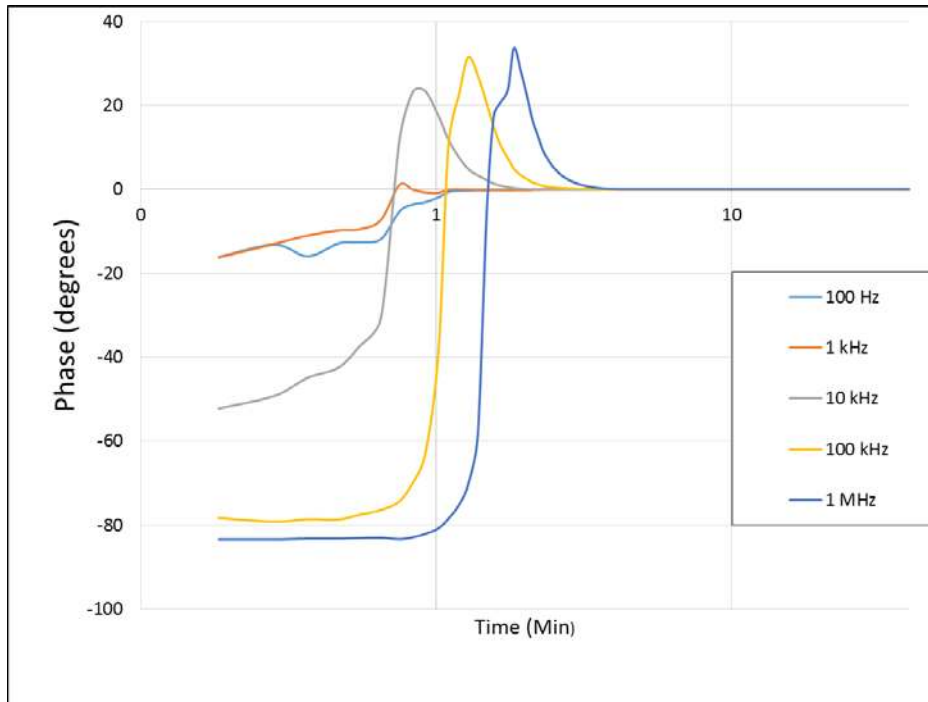
Figure 13 The phase measurement during cure at 95°C for GEM 2
