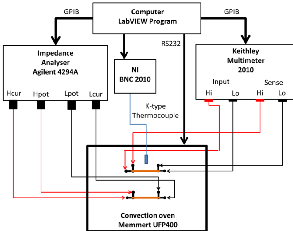
Figure 4 Block diagram of the test setup for electrical measurement
