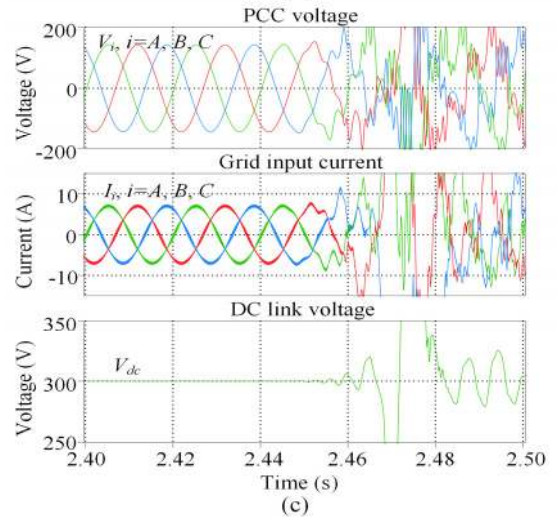
Fig. 14. Simulated waveforms of VSC in the rectifier mode. (a) k_p=0.5 . (b) k_p=1.4 . (c) k_p=2.0 .
