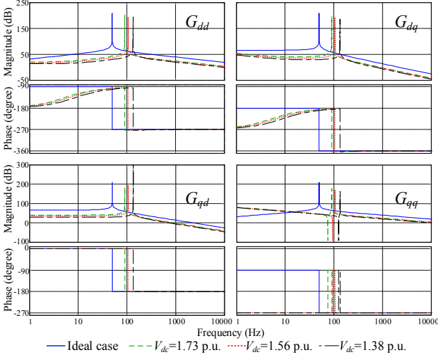
Fig. 5. Frequency response of four channels of L -filter plant and \mathbf{G}_{p-ac} different dc-link voltage levels.
