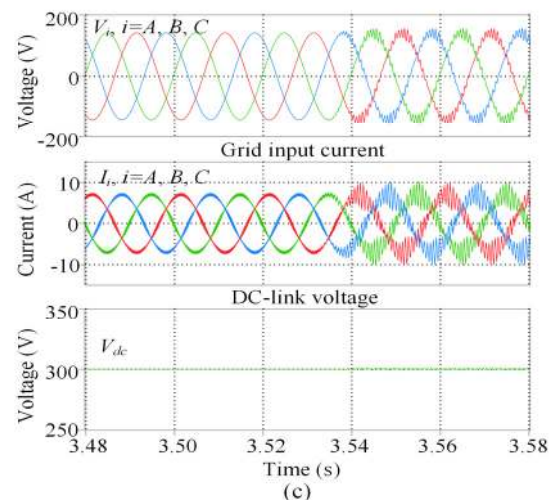
Fig. 16. Simulated waveforms of VSC in the inverter mode. (a) k_p=0.5 . (b) k_p=1.5 . (c) k_p=2.0 .
