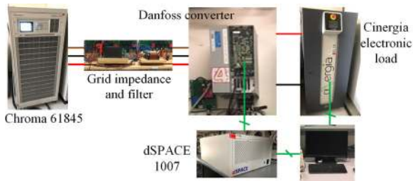
Fig. 18. Experimental setup in the lab.
