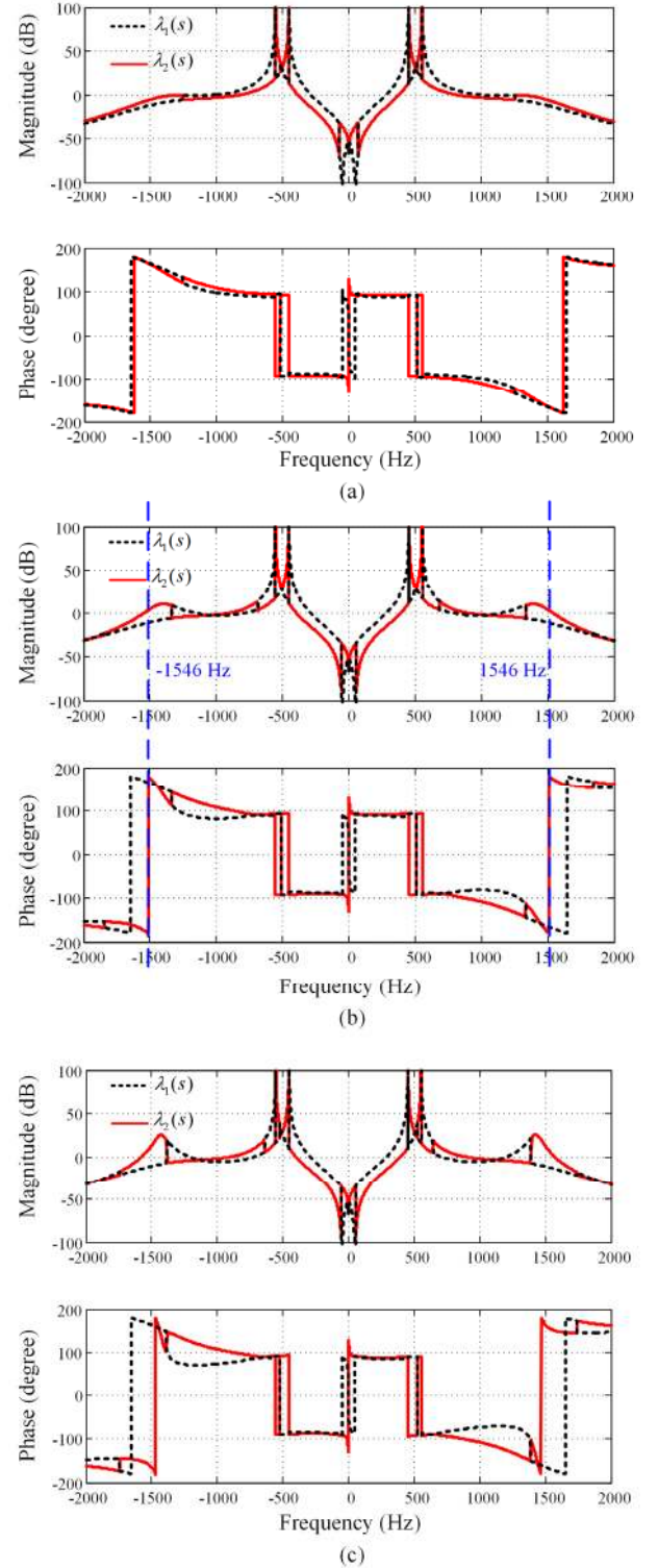
Fig. 12. Frequency response of the eigenvalues in the inverter mode. (a) k_p=0.5 . (b) k_p=1.5 . (c) k_p=2.0 .
