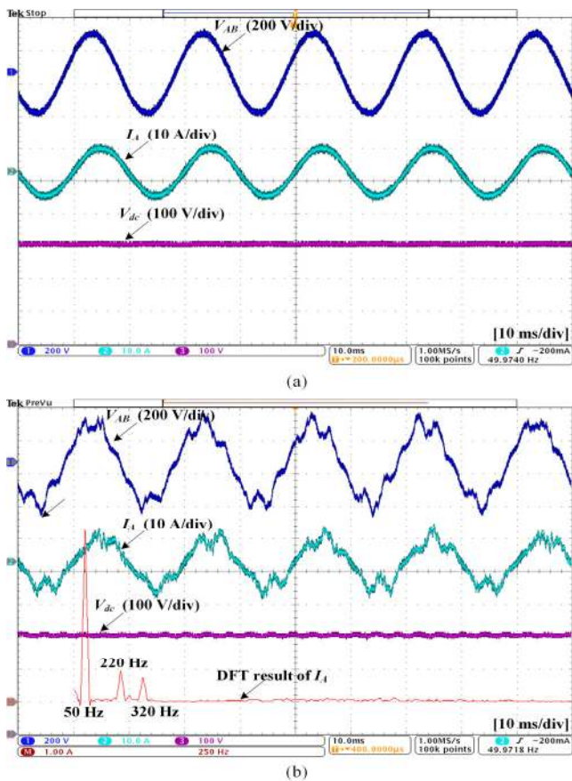
Fig. 19. Experimental waveforms of the PCC voltage, input current and dc-link voltage in the rectifier mode. (a) k_p=0.5 . (b) k_p=1.4 .
