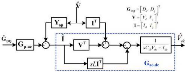
Fig. 4. Small-signal model of dc-link dynamics \mathbf{G}_{p-dc} .
