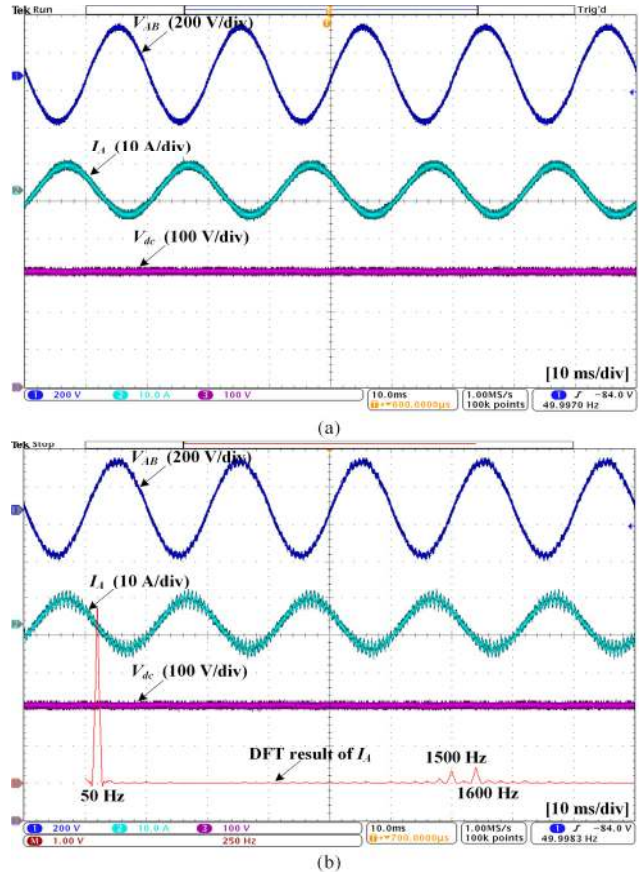
Fig. 20. Experimental waveforms of the PCC voltage, input current and dc-link voltage in the inverter mode. (a) k_p=0.5 . (b) k_p=1.5 .
