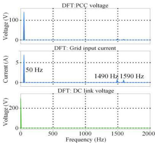
Fig. 17. Harmonic spectrum of the simulated waveforms in Fig. 16(b).
