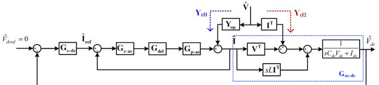
Fig. 8. Block diagram of the transfer function matrices of the VSCs with cascaded control loops.
