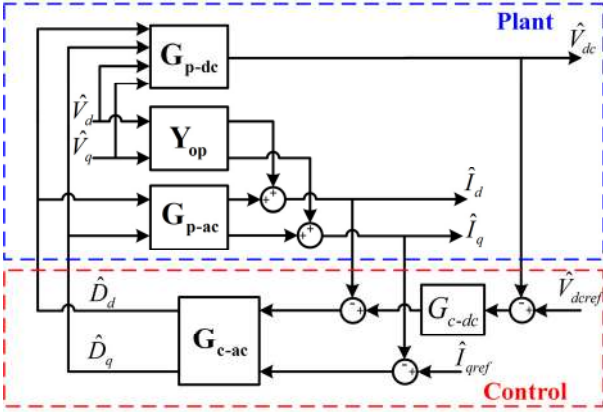
Fig. 3. Small-signal model of the VSC.
