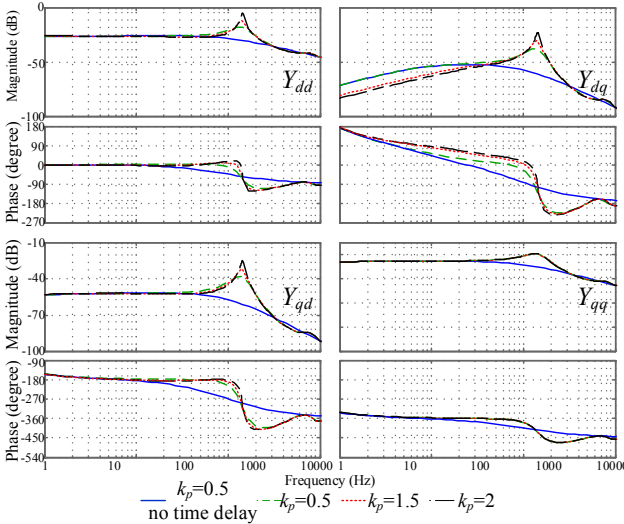
Fig. 10. Input admittance \mathbf{Y}_{cl} of inverter mode represented in the dq -frame.
