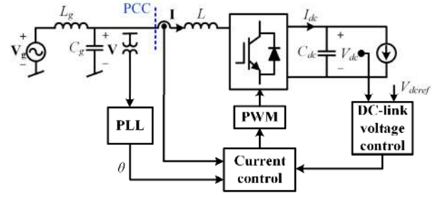
Fig. 1. Single-line circuit diagram and control system of a three-phase VSC.
