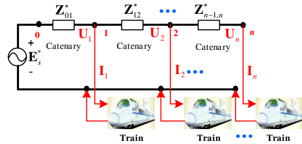
Fig. 7. A typical configuration of the MTNS.
