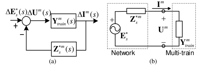
Fig. 8. Multi-train modeling (a) block diagram of multivariable feedback system; (b) Thevenin representation of the MTNS.
