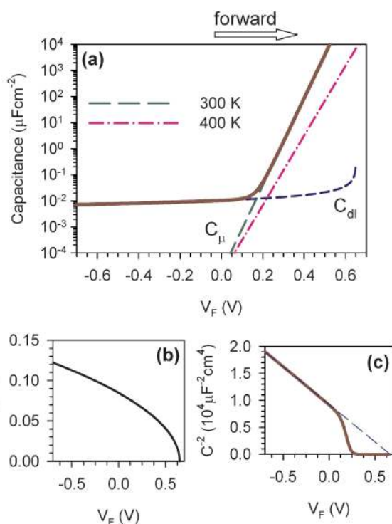
Fig. 4 Theoretical calculation of: (a) capacitances in the solar cell: chemical capacitance C_{\mu} (calculated at two different temperatures, as indicated), capacitance in the depletion layer C_{\text{dl}} , and total capacitance (thick line). (b) Width of the space charge region. (c) Mott–Schottky plot. Parameters used in the simulation: L = 300 \mu\text{m} , T = 300 \text{K} , V_{\text{bi}} = 0.65 \text{V} , \epsilon_r = 1 , N_A = 10^{16} \text{cm}^{-3} , n_0 = 1 \times 10^8 \text{cm}^{-3} .
