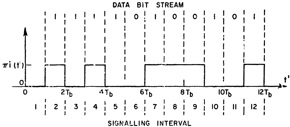
Fig. 1. A differential encoding example.
