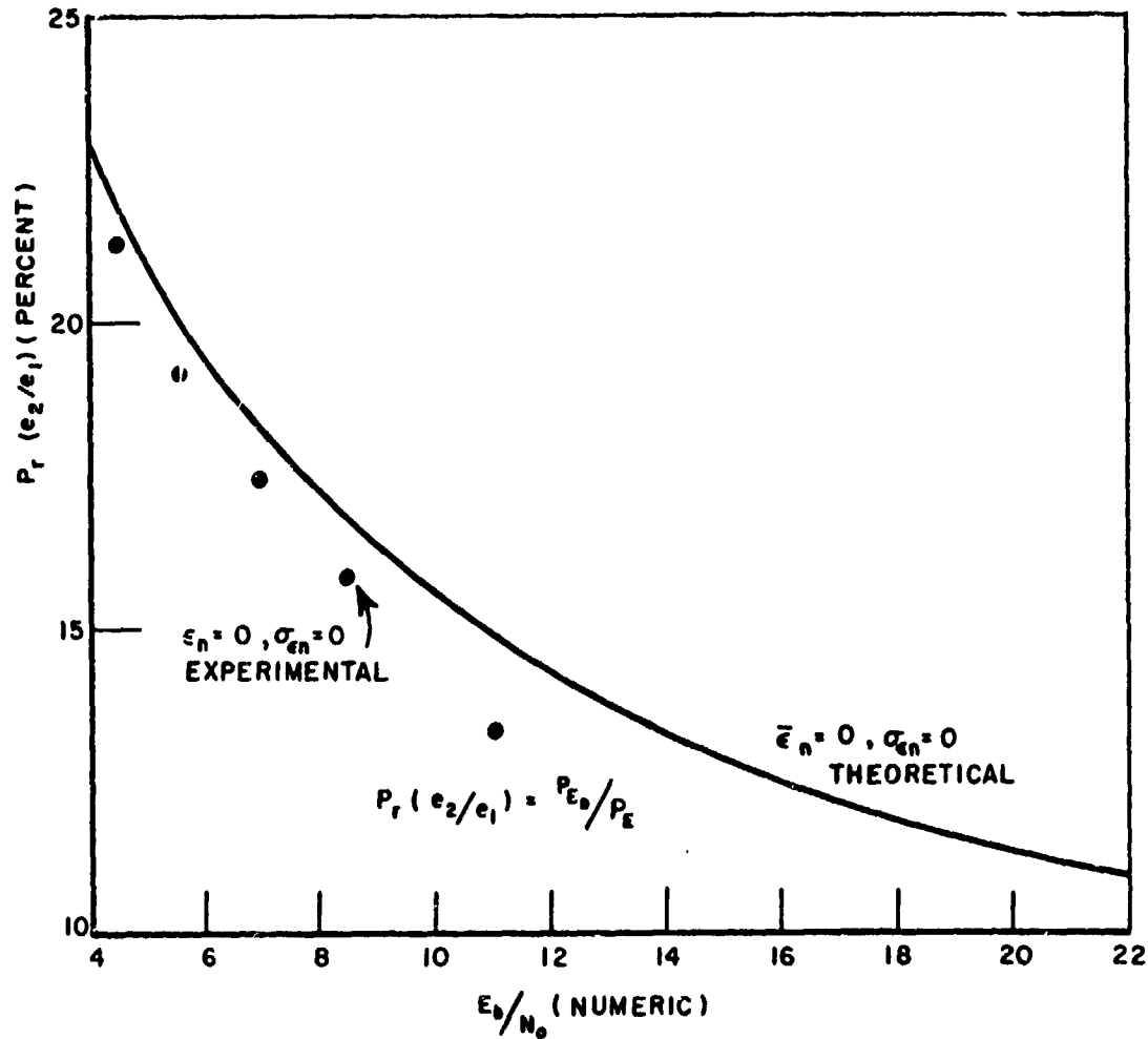
Fig. 18. The probability of error given that an error was detected in the previous bit interval versus the bit energy to noise density ratio for \epsilon = 0 , \sigma_{\epsilon} = 0 and \Delta f_0 = 0 ; both analytical and experimental results are given.
