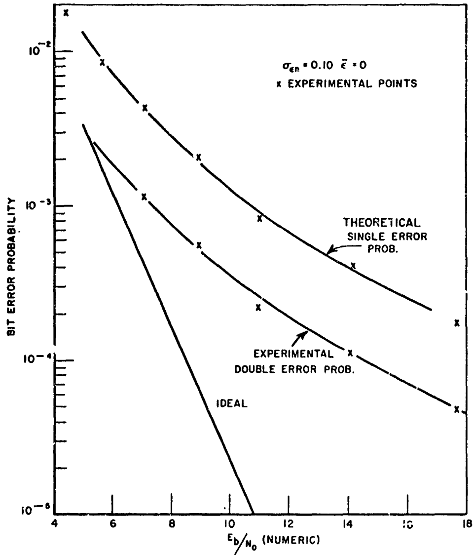
Fig. 21. The bit error probability versus the bit energy to noise density ratio for the imperfectly-timed DD; \bar{\epsilon}_n=0 and \sigma_{\epsilon n}=0.10 . Both analytical and experimental results are given. Nominal experimental results for the probability of two consecutive errors are also given.
