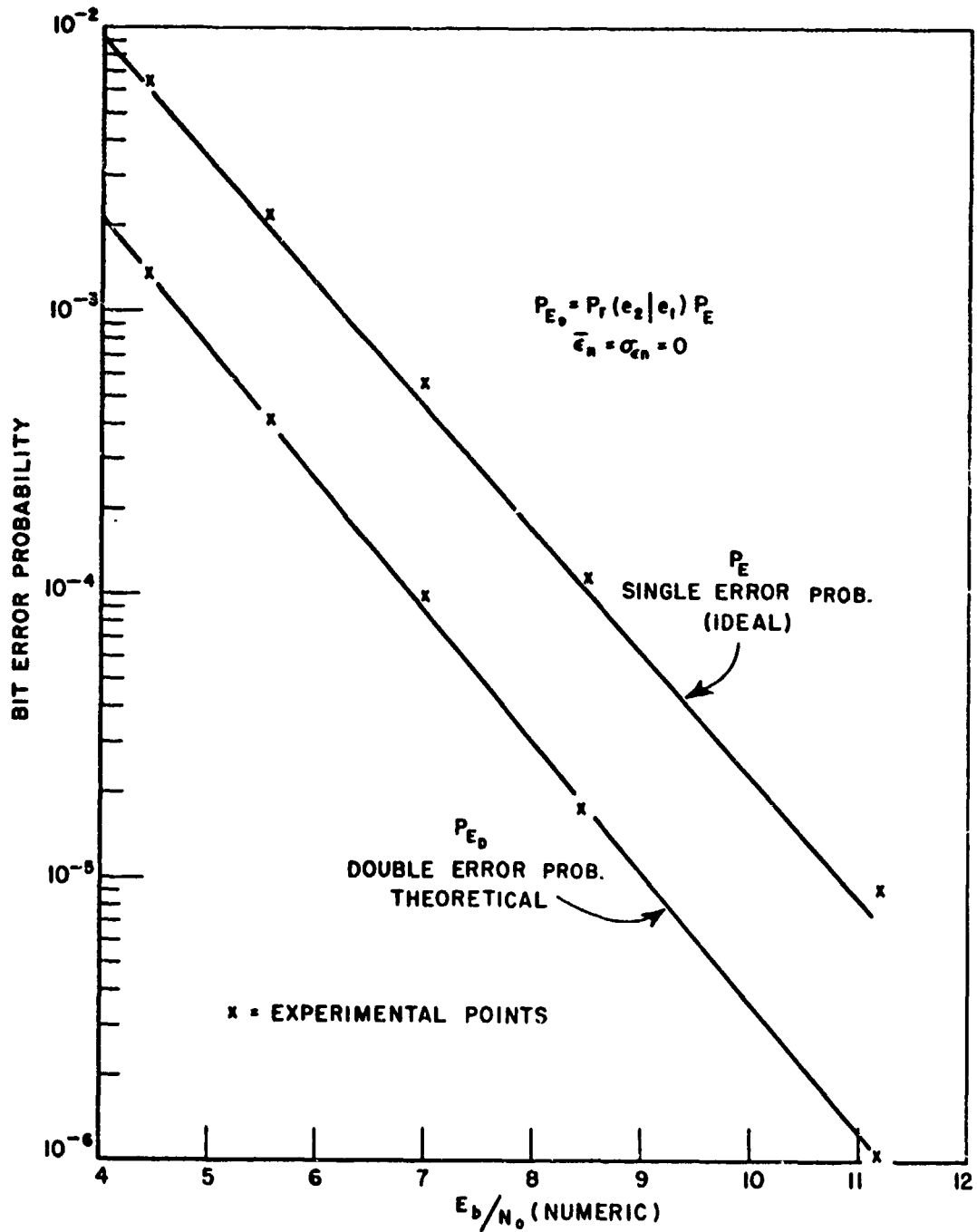
Fig. 17. The bit error probability versus the bit energy to noise density ratio under best case conditions; \epsilon=0 , \sigma_\epsilon=0 and \Delta f_0=0 . Both analytical and experimental results are given. Analytical and experimental results for the probability of two consecutive errors are also given.
