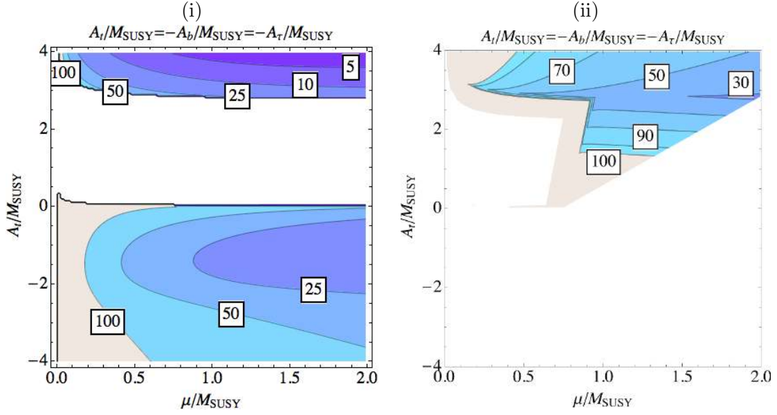
Figure 4. Same as figure 3 but now showing alignment values of t_\beta under the assumptions A_b = A_\tau = -A_t .
