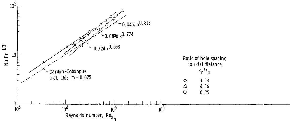
(b) Test results of reference 23 compared to results of reference 16. Wall temperature T_w = 339 K (150° F).
