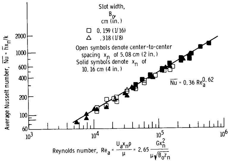
Figure 17. - Correlation of average heat-transfer coefficients between a plate and arrays of impinging two-dimensional jets. Mass flow rate per jet exit area G = 977 to 7812 kg/(hr)(m 2 ), or 200 to 1600 lb/(hr)(ft 2 ); dimensionless nozzle-to-plate spacing z_n/B_0 = 8 to 64 . (From ref. 27.)
