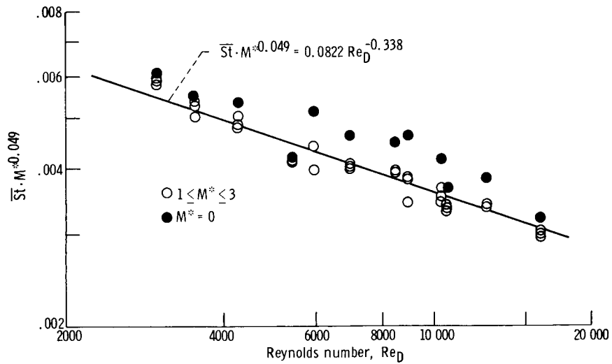
Figure 11. - Empirical correlation of the overall effect of crossflow for a row of holes. Dimensionless nozzle-to-plate spacing z_n/D = 2 ; ratio of unheated starting length to nozzle diameter L/D = \pm 10 ; dimensionless hole spacing, 2.5 \leq x_n/D \leq 5.0 . (From ref. 26.)
