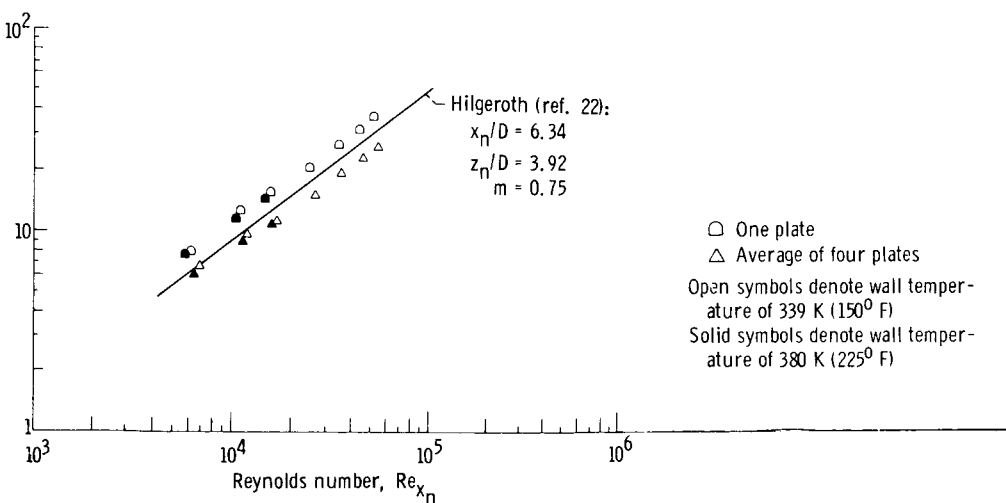
(c) Test results of reference 23 compared to results of reference 22.
