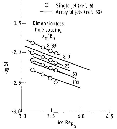
Figure 18. - Single-slot-jet results (ref. 6) compared with results for arrays of slot jets (ref. 30). Dimensionless nozzle-to-plate spacing z_n/B_0 = 8 . (From ref. 30.)
