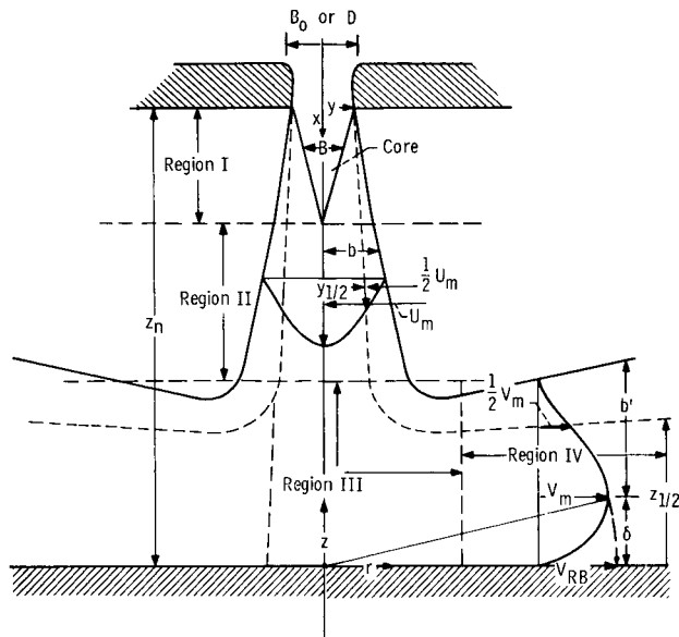
(a) Characteristic regions in impinging jet flow. (From ref. 1.)
