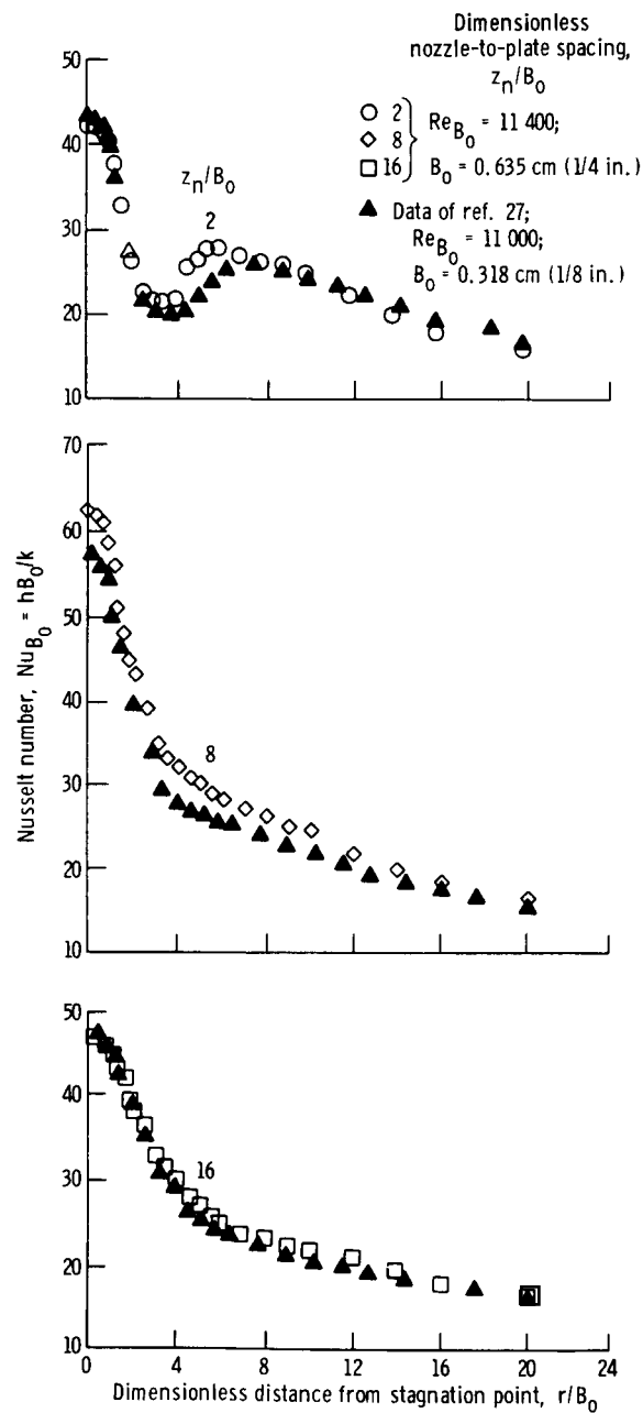
Figure 14. - Comparison of local Nusselt number measurements for a slot jet with those of reference 27. (From ref. 9.)
