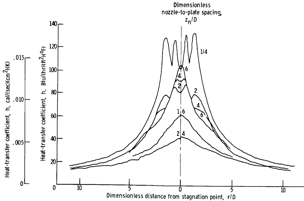
Figure 4. - Radial variation of heat transfer between a plate and an impinging jet. Nozzle diameter D = 0.634 centimeter (0.250 in.); Re_D = 28\,000 ; temperature difference \Delta T = 20\text{ K} ( 36^\circ\text{ F} ). (From ref. 16.)
