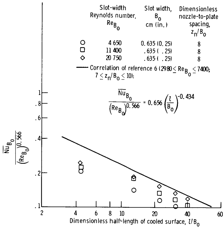
Figure 15. - Comparison of average heat-transfer data for a slot jet with empirical correlation of reference 6. (From ref. 9.)
