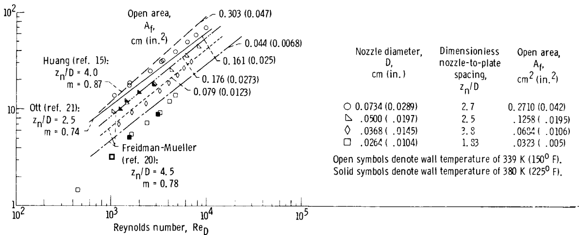
(a) Test results of reference 23 compared to results of references 15, 20, and 21. Constant hole spacing, x_n = 0.318 centimeter (0.125 in.); jet temperature, 297 K (75° F).
