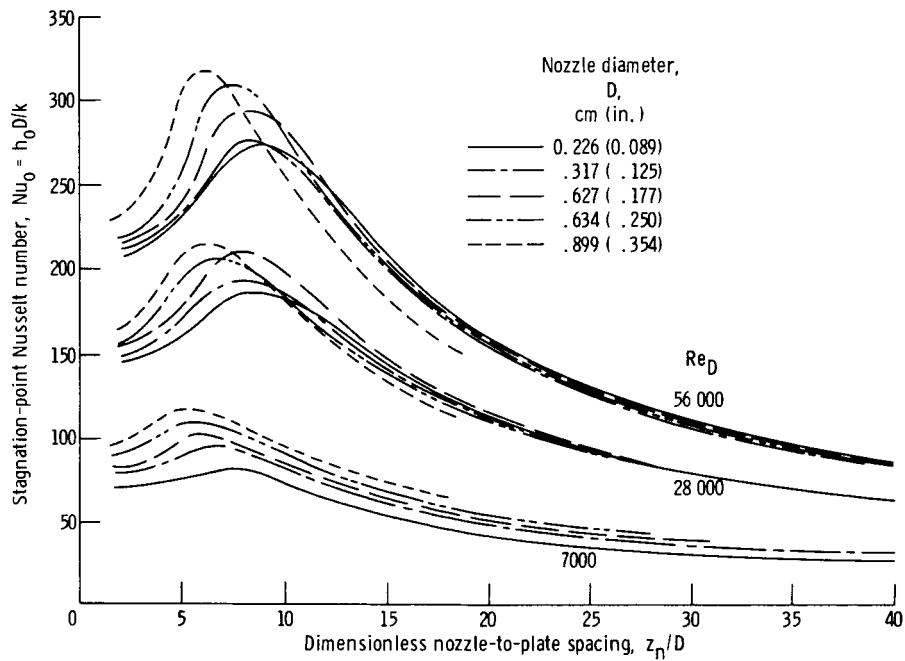
Figure 3. - Correlation of heat-transfer coefficient at stagnation point of a jet. (From ref. 16.)
