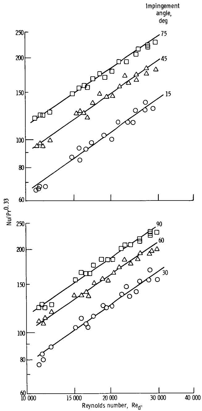
Figure 2. - Effect of impingement angle on heat transfer. (From ref. 13.)
