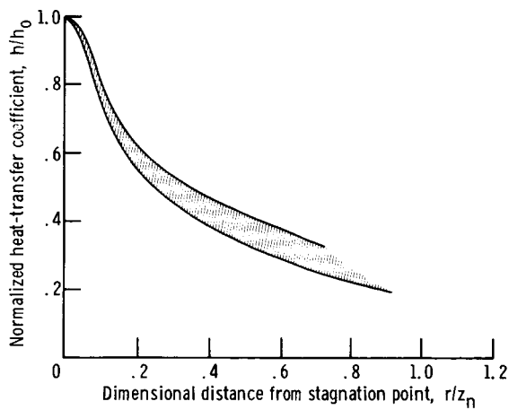
Figure 5. - Radial variation of normalized heat-transfer coefficients between a plate and an impinging jet. Dimensionless nozzle-to-plate spacing z_n/D > 10 ; Re_D > 7000 . (From ref. 16.)
