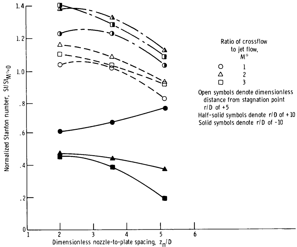
Figure 9. - Effect of nozzle-to-plate spacing on normalized Stanton number for row of holes with center-to-center hole spacing of three hole diameters. Dimensionless hole spacing x_n/D = 3.0 ; equivalent-slot Reynolds number Re_{eS} = 2000 . (From ref. 26.)
