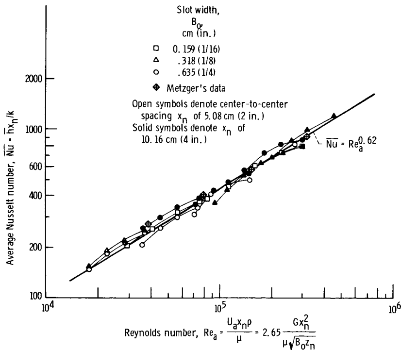
Figure 13. - Correlation of average heat-transfer coefficients between a target of finite width and a single two-dimensional air jet. Mass flow rate per jet exit area G = 3515 to 28\ 123 kg/(hr)(m 2 ), or 720 to 5760 lb/(hr)(ft 2 ); dimensionless nozzle-to-plate spacing z_n/B_0 = 8 to 64 . (From ref. 27.)
