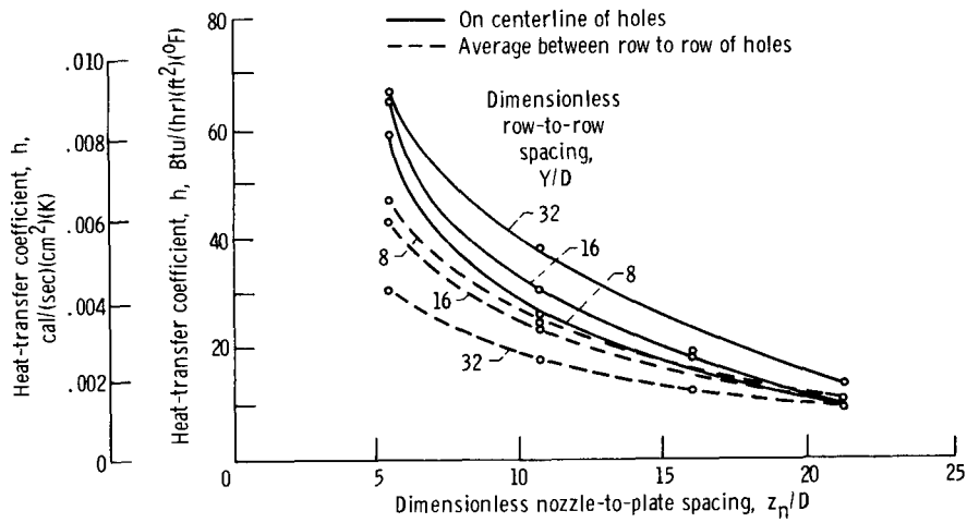
Figure 7. - Variation of heat-transfer coefficient under simple multiple jets with axial distance ratio z_n/D . Nozzle diameter D = 0.476 centimeter (3/16 in.); center-to-center spacing x_n = 1.588 centimeters (5/8 in.); row-to-row spacing Y = 3.81, 7.62, 15.24 centimeters (1.5, 3, 6 in.). (From ref. 15.)
