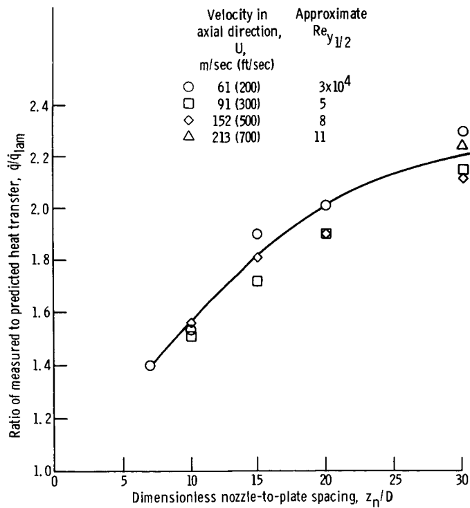
Figure 6. - Ratio of measured heat transfer to that predicted by laminar theory at stagnation point of impinging jet. (From ref. 18.)
