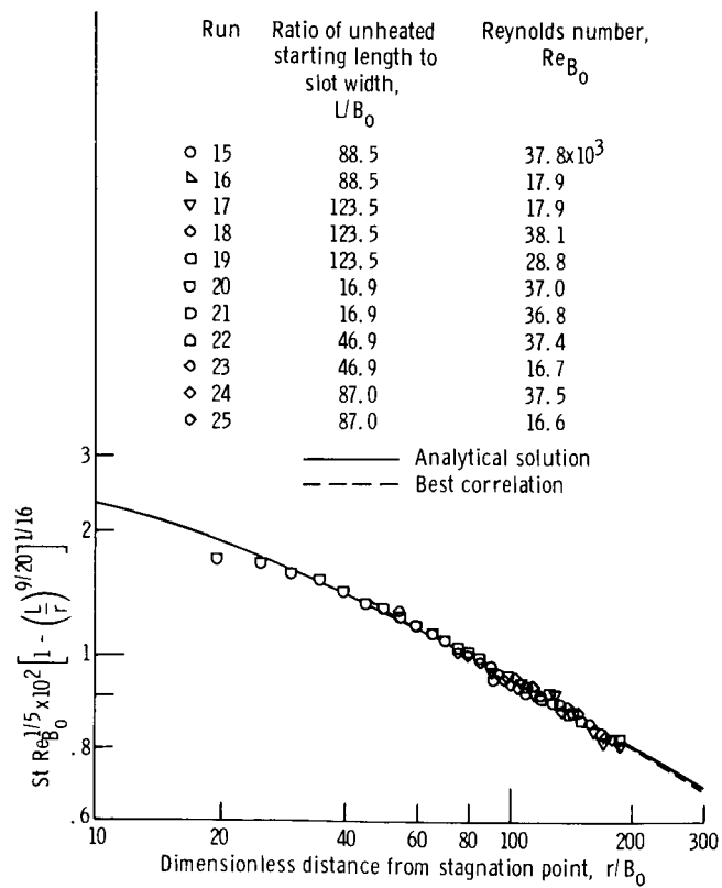
Figure 12. - Heat transfer to wall jets from an isothermal wall with an unheated starting length (correlated data). (From ref. 8.)
