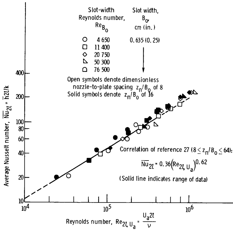
Figure 16. - Comparison of average heat-transfer data for a slot jet with empirical correlation of reference 27. (From ref. 9.)
