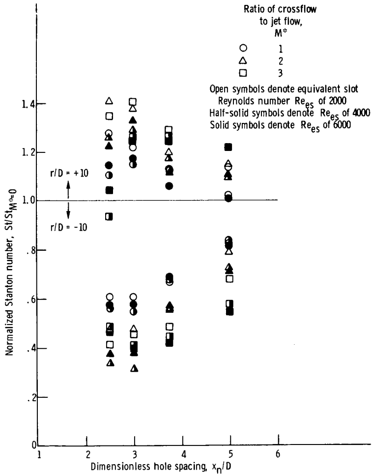
Figure 10. - Effect of center-to-center hole spacing on normalized Stanton number for a row of holes with nozzle-to-plate spacing of 2 nozzle diameters. (From ref. 26.)
