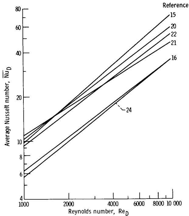
Figure 19. - Nusselt number as function of Reynolds number for two-dimensional array of circular jets as calculated from references 15, 16, 20, 21, 22, and 24. (From ref. 31.)
